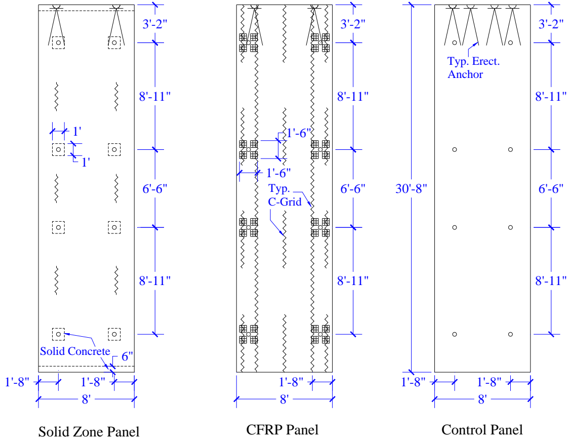
Figure 1: Wall Elevations
