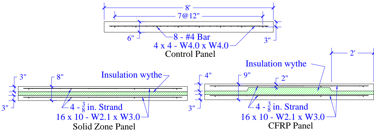
Figure 2: Wall Sections
