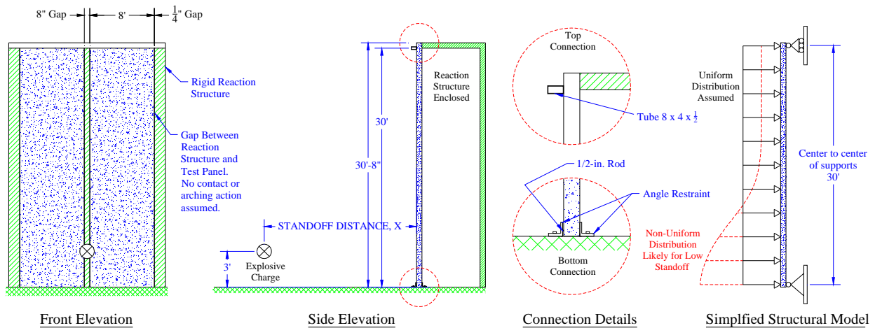
Figure 4: Loading configuration
