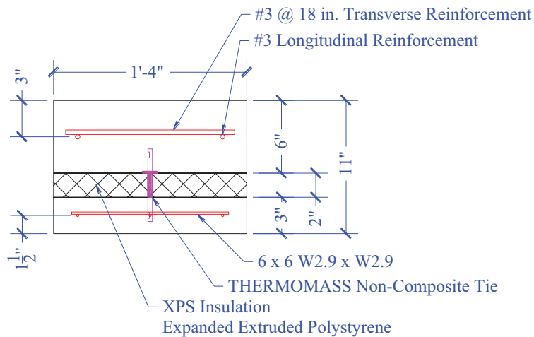
Figure 180. TS3-A, B Cross-Section Detail
