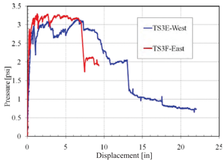
Figure 214. Measured Responses
