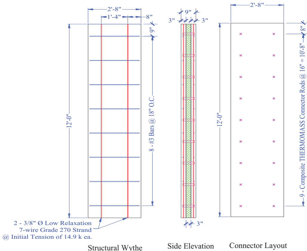
Figure 118. PCS8 Panel Detail
