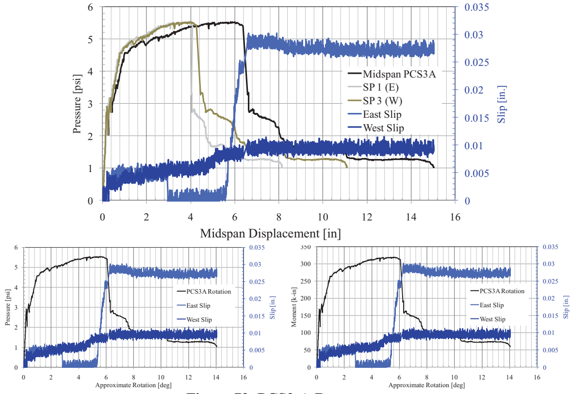
Figure 72. PCS3-A Response
