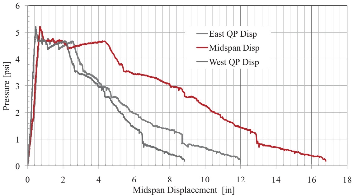
Figure 138. Tyn1-C Response
