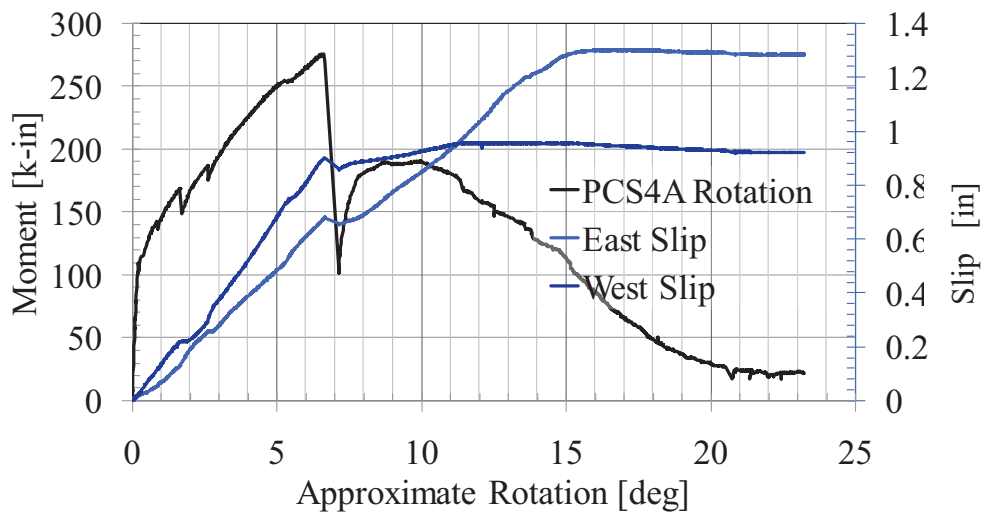
Figure 89. PCS4-A Response
