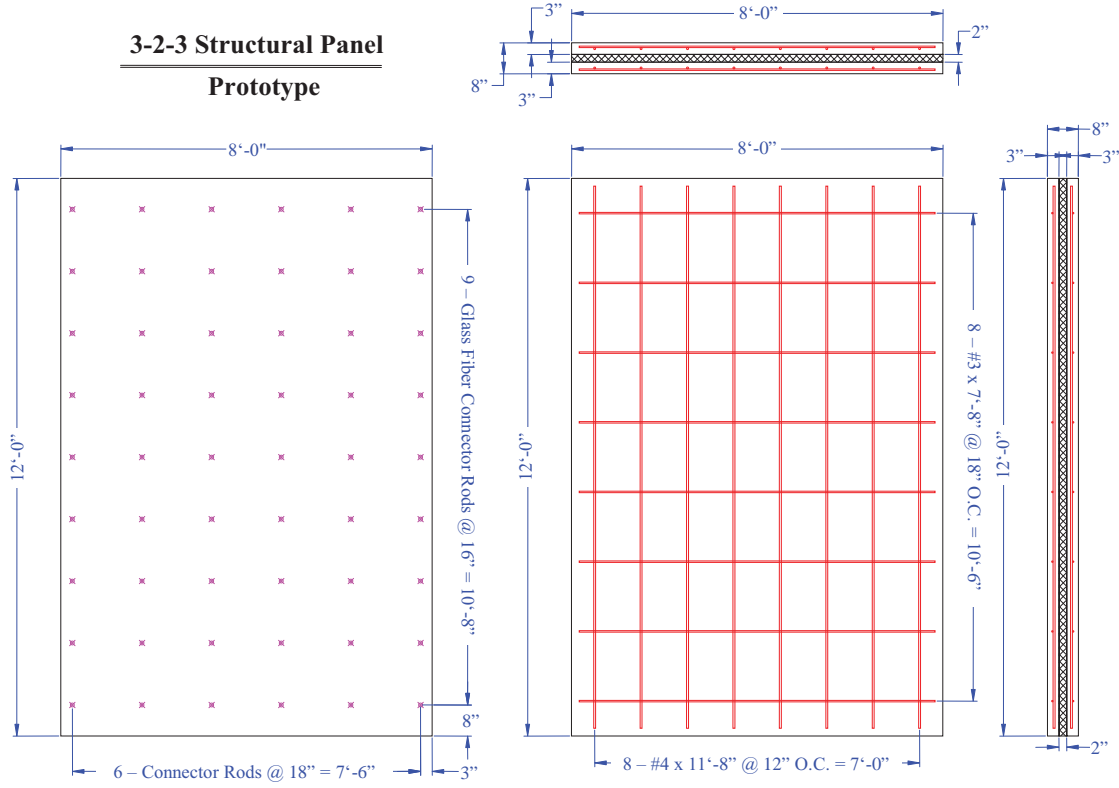
Figure 6. Prototype TCA 3-2-3 Wall
