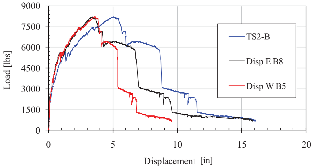
Figure 49. TS2-B Detail Results
