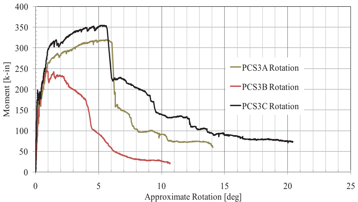
Figure 71. PCS3 Moment-Rotation Response
