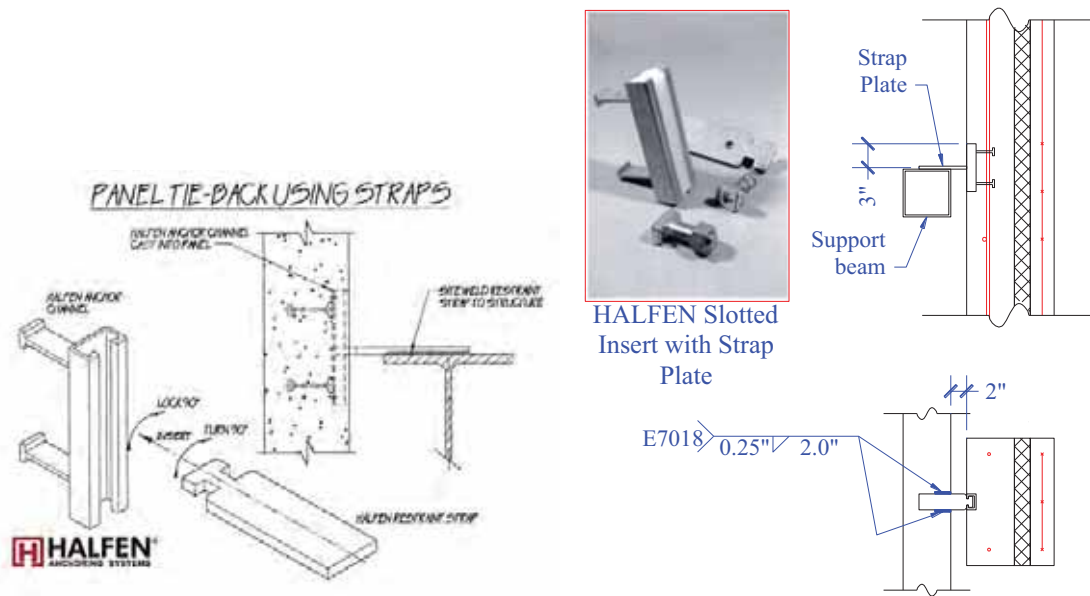
Figure 21. TS3-A and B Connection Details
