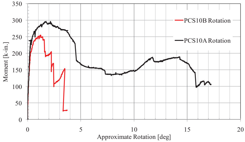
Figure 148. PCS10 Moment–Rotation Response
