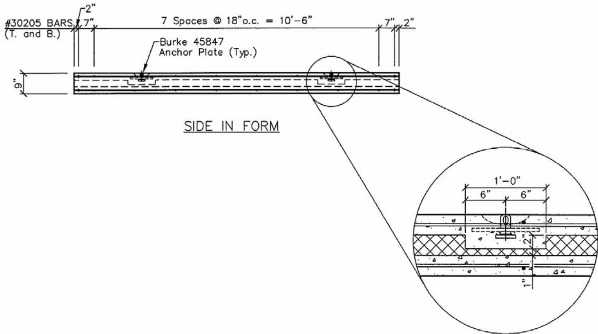
Figure 86. PCS4 Panel Detail 2
