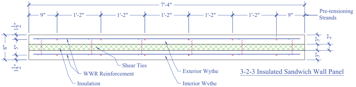
Figure 1. Sandwich Panel Cross-Section
