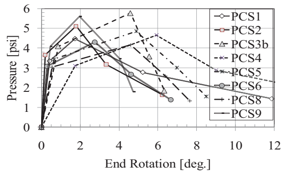
Figure 212. Prestressed Backbones
