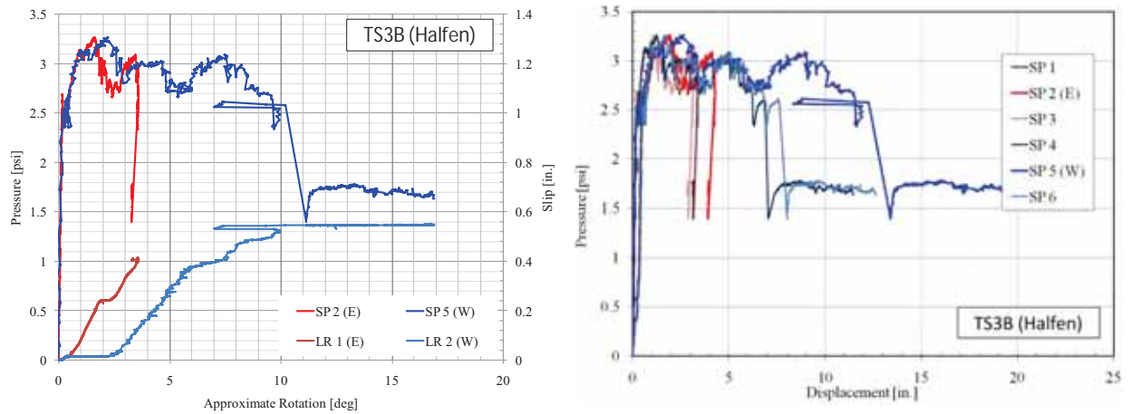
Figure 185. TS3-B Response
