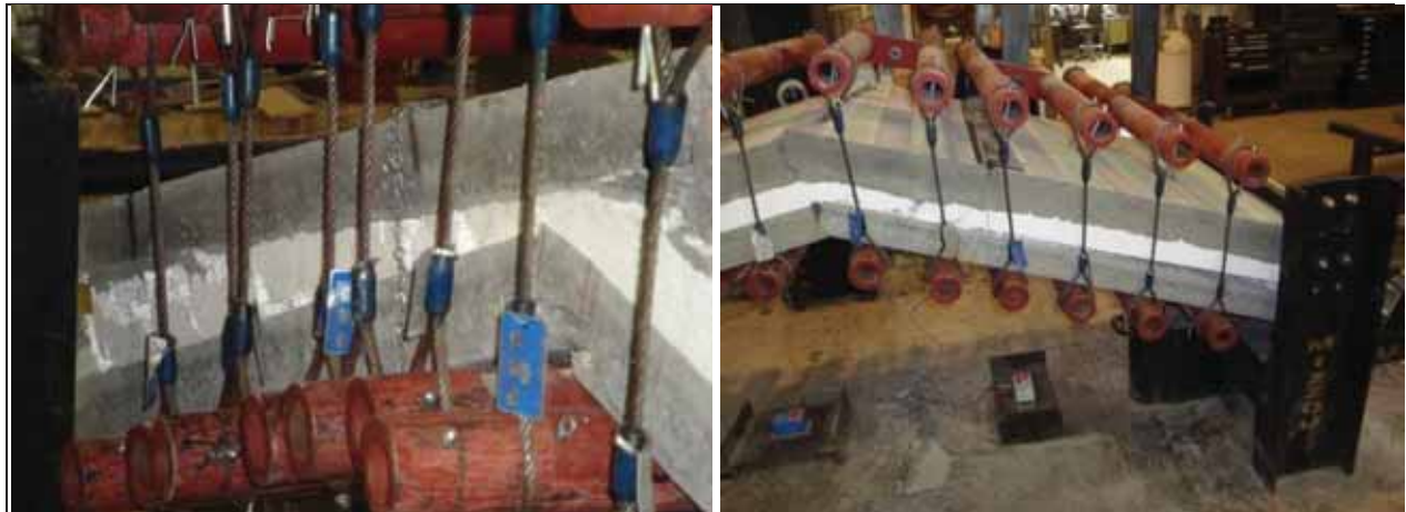
Figure 108. PCS6 Panel Response (A, B)
