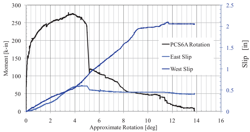
Figure 105. PCS6-A Response
