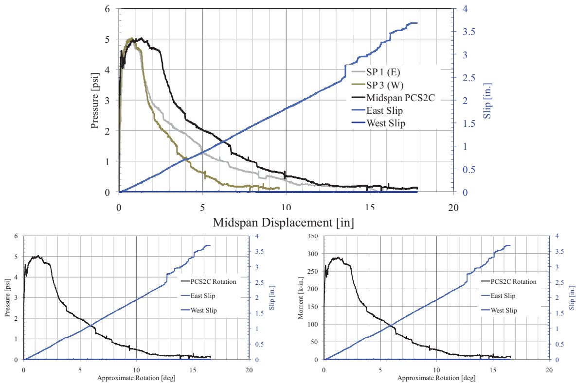
Figure 66. PCS2-C Response
