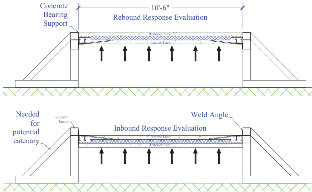
Figure 35. Schematic of End Connection Setup
