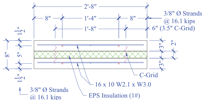
Figure 60. PCS2 Cross-Section Detail
