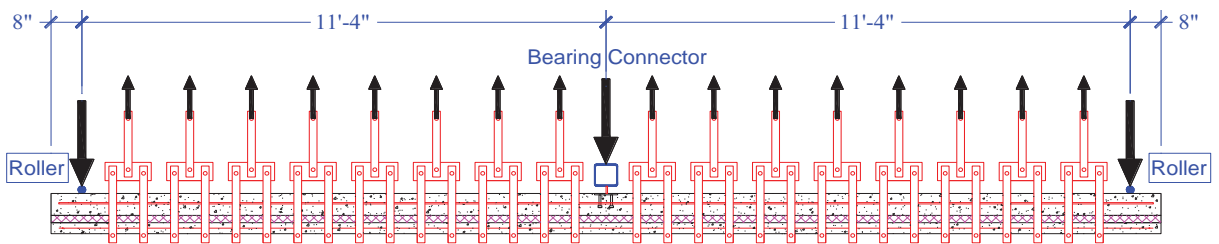
Figure 34. Schematic of Single and Two-span Fixtures
