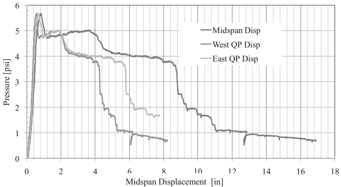
Figure 142. Tyn2-A Response
