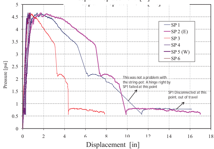
Figure 178. PCD2-C Response
