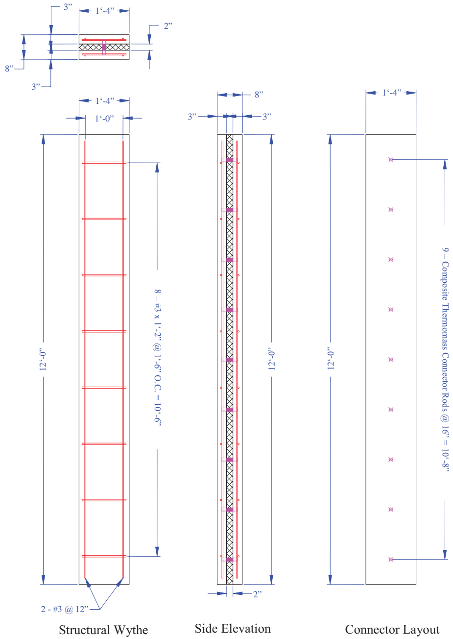
Figure 9. TCA Composite 3-2-3 Single-span Static Specimen TS2 Details
