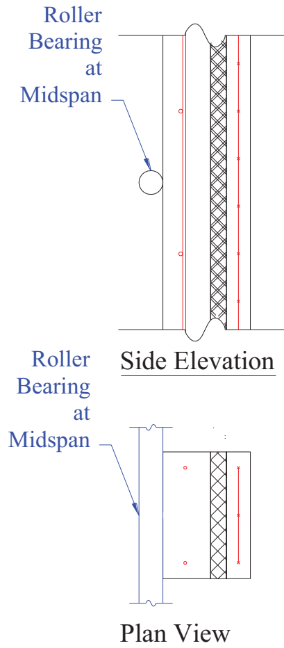
Figure 189. TS3-C, D Connection Detail
