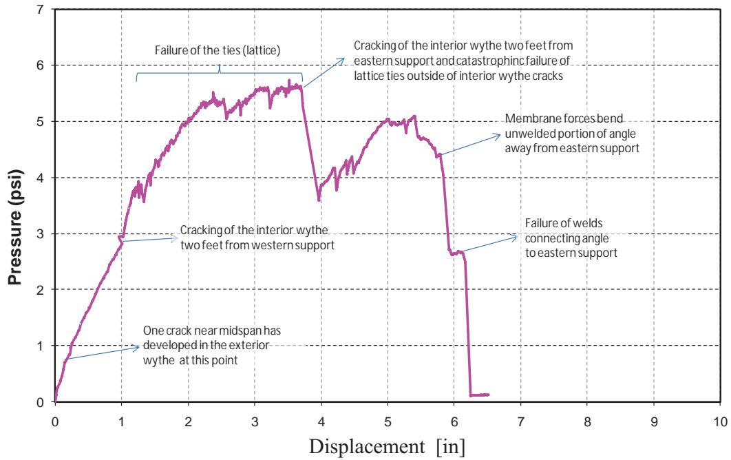
Figure 158. PCS11-B Response
