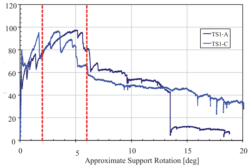
Figure 40. TS1 6-2-3 Moment—Rotation
