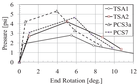
Figure 211. Reinforced Backbones
