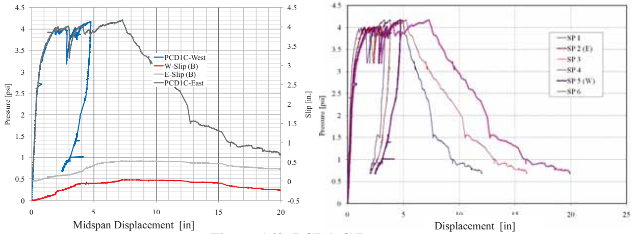
Figure 169. PCD1-C Response
