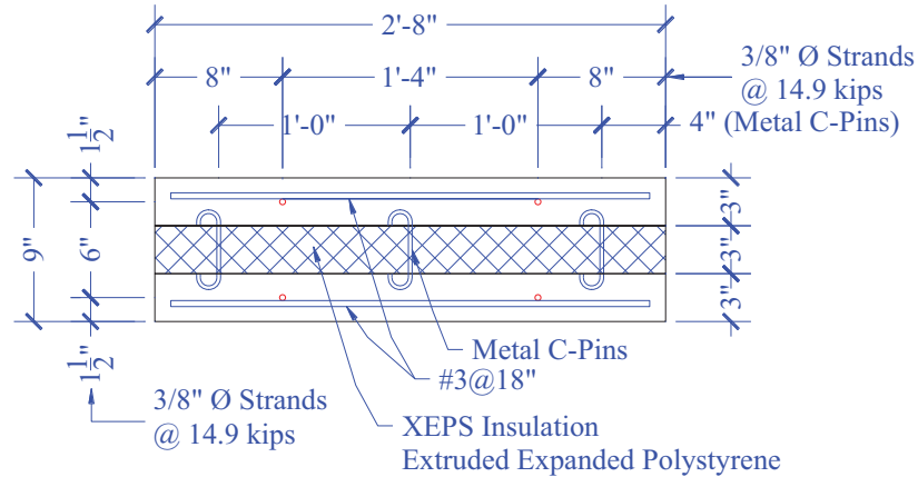
Figure 84. PCS4 Cross-Section Detail
