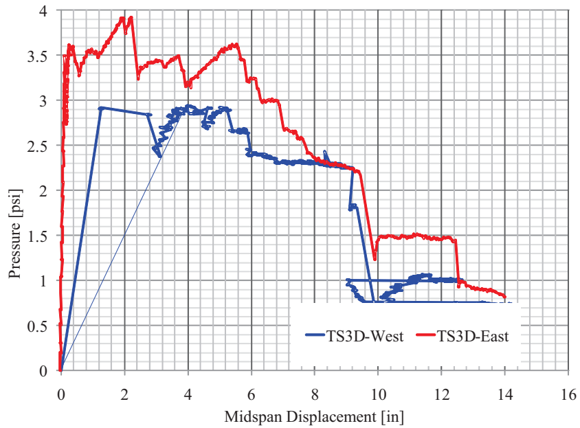
Figure 190. TS3-C, D Pressure-Displacement Response
