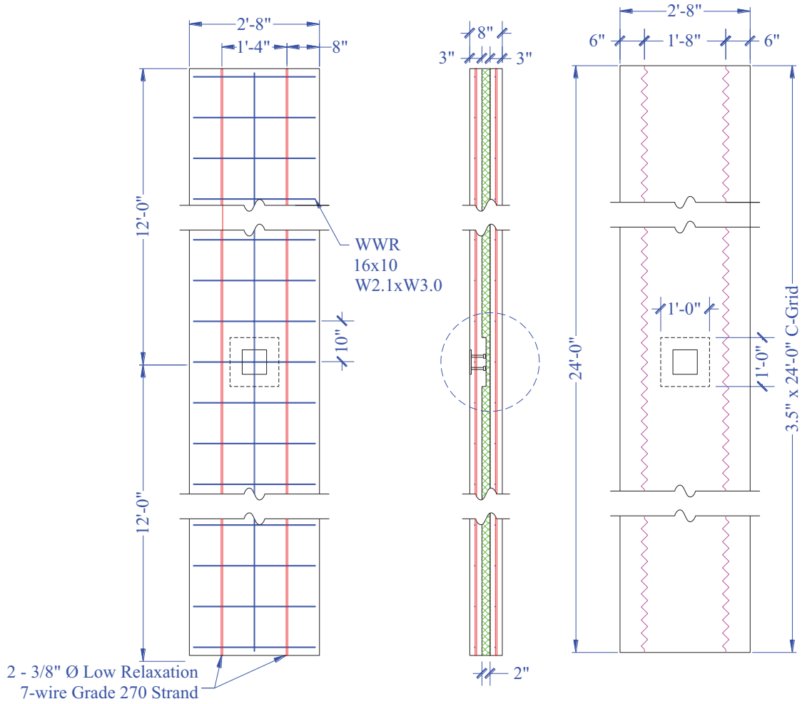
Figure 19. Metromont Two-span Panel PCD2
