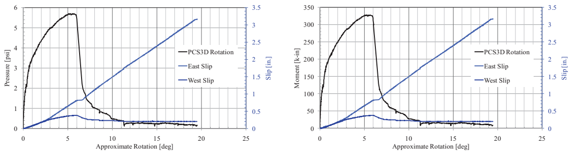
Figure 80. PCS3-D Response
