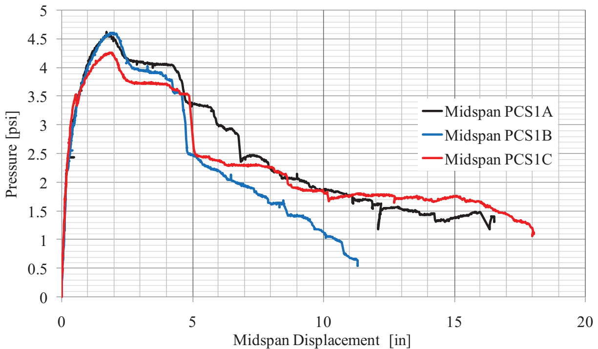
Figure 54. PCS1 Pressure–Displacement Response
