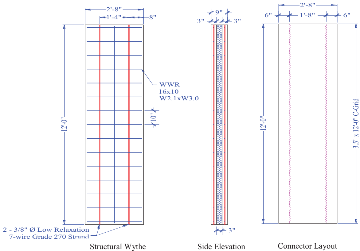
Figure 102. PCS6 Panel Detail
