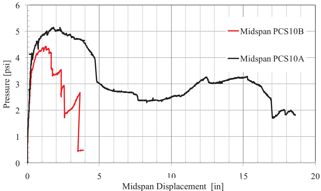
Figure 147. PCS10 Pressure–Displacement Response
