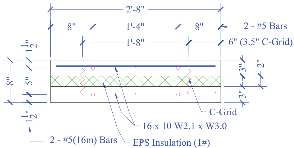
Figure 68. PCS3 Cross-Section Detail
