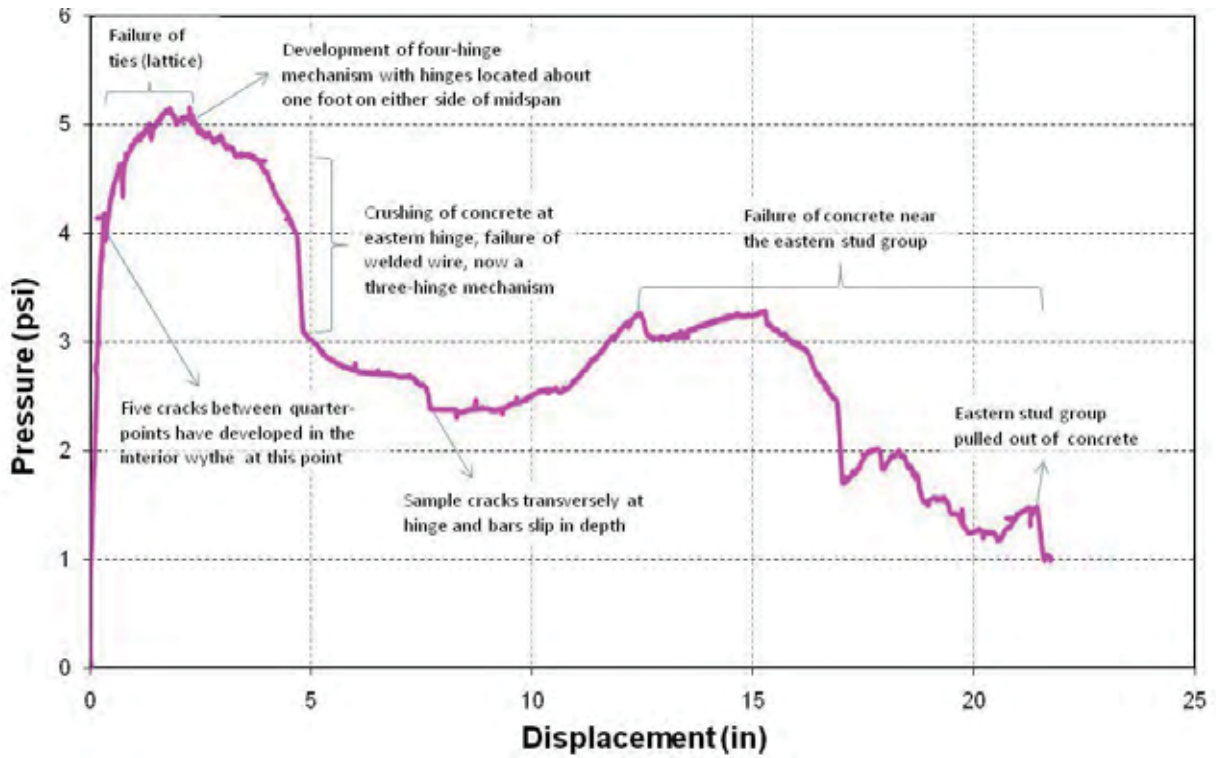
Figure 149. PCS10-A Inbound Response
