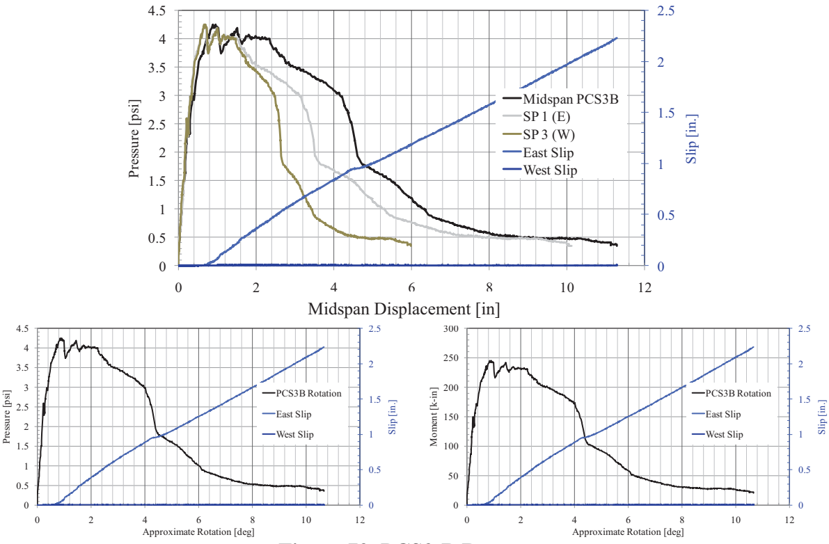
Figure 73. PCS3-B Response
