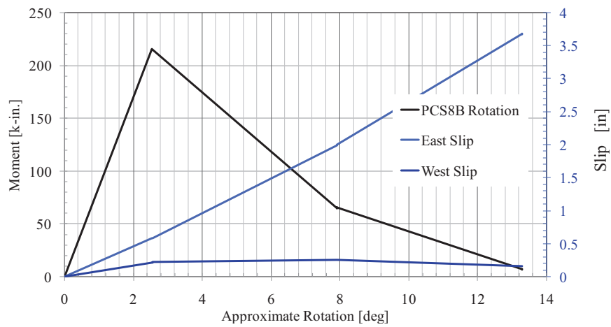
Figure 122. PCS8-B Response
