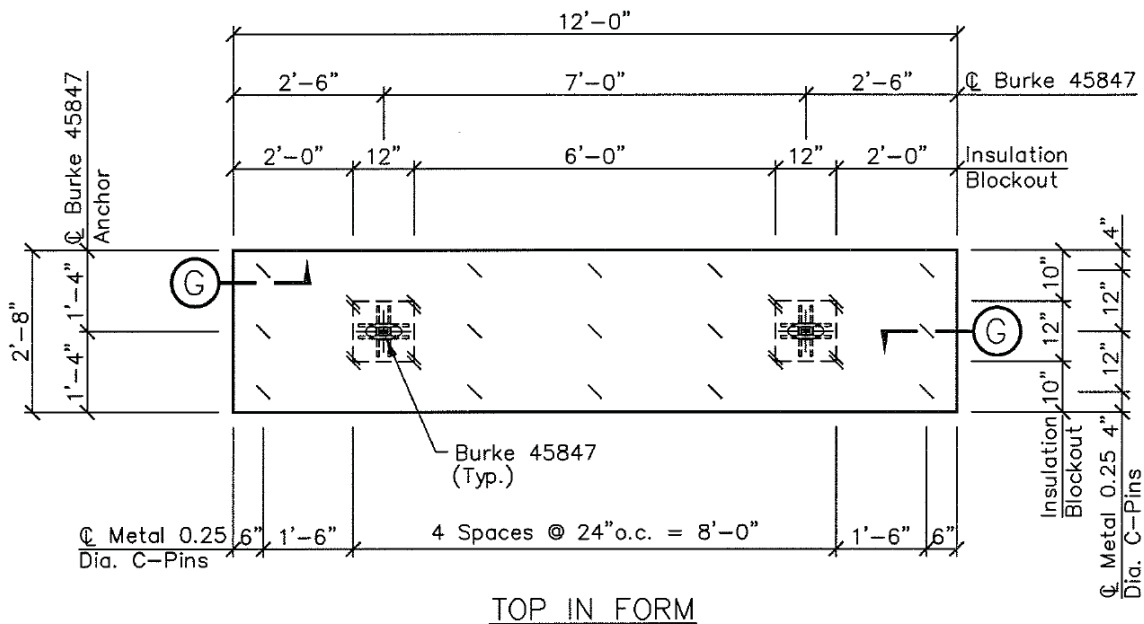
Figure 85. PCS4 Panel Detail
