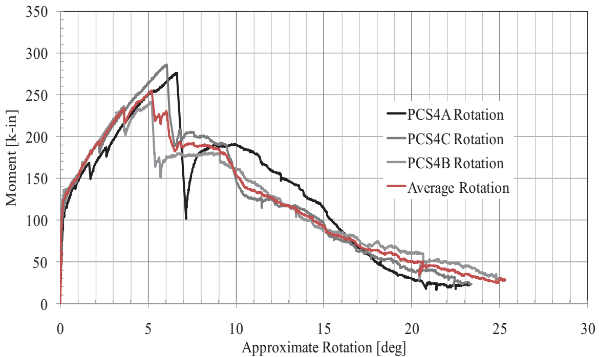
Figure 88. PCS4 Moment-Rotation Response
