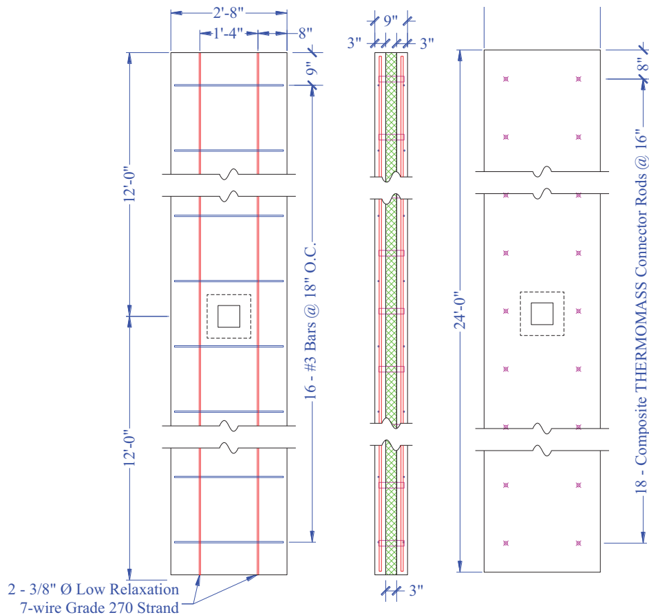
Figure 162. PCD1 Panel Detail
