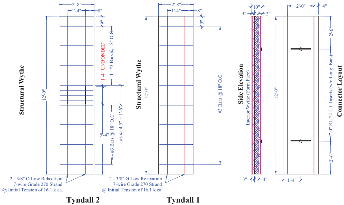
Figure 14. Tyndall Panel Reinforcement
