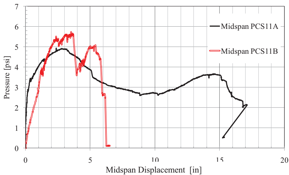
Figure 155. PCS11 Pressure–Displacement Response
