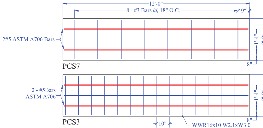
Figure 13. Control Panel Reinforcement
