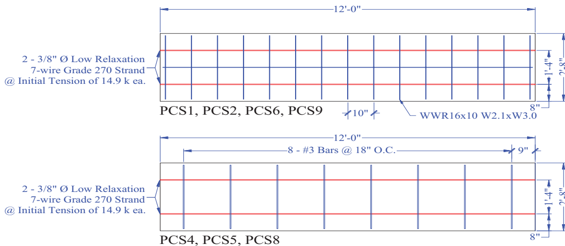
Figure 12. PCI Panel Reinforcement
