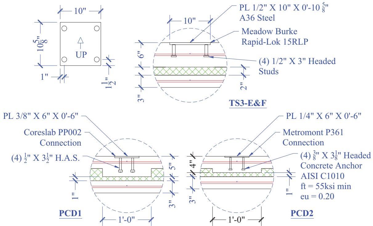
Figure 23. Connection Details for PCI Panels PCD1 and PCD2
