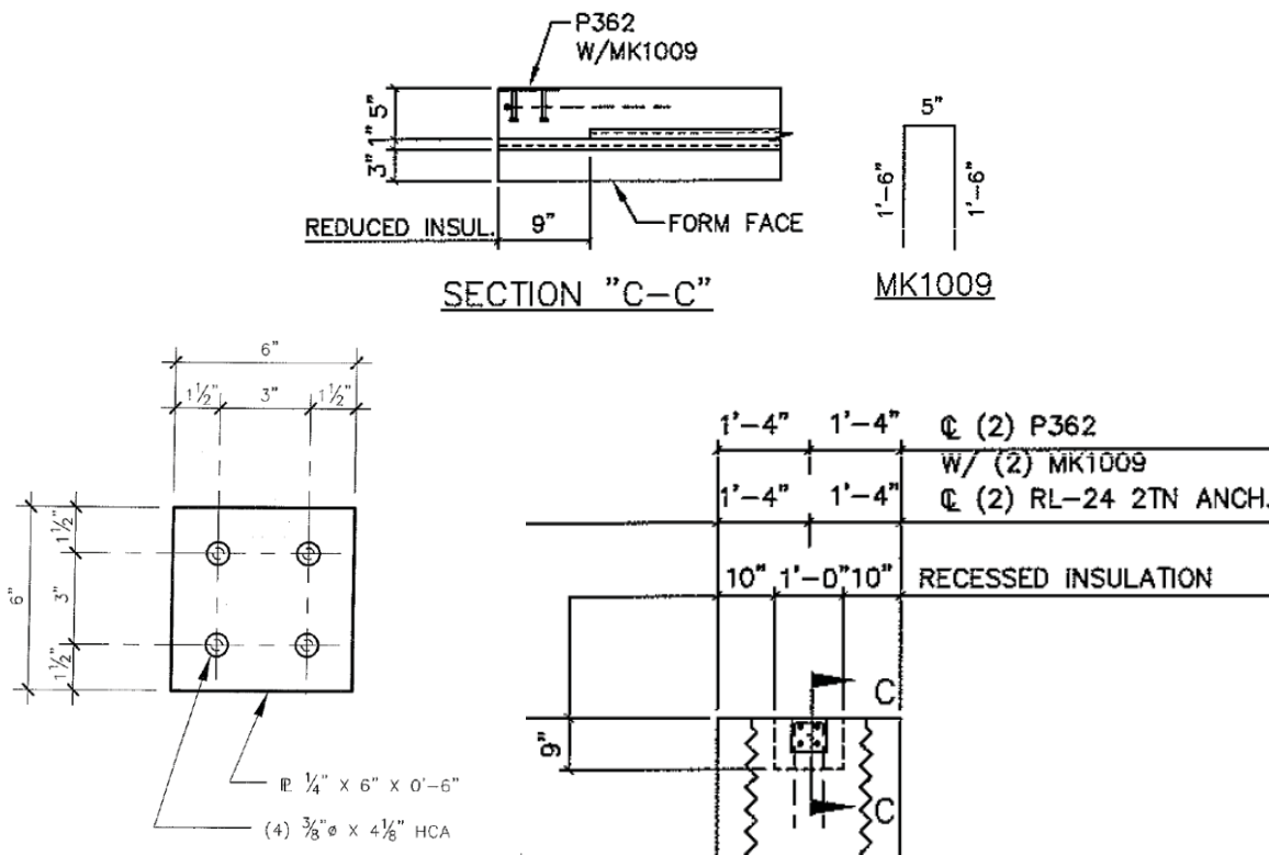
Figure 28. PCS10 Connection Details
