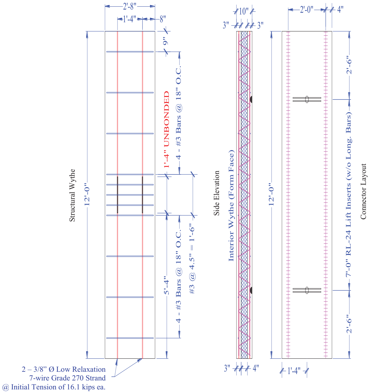
Figure 140. Tyn2 Panel Detail
