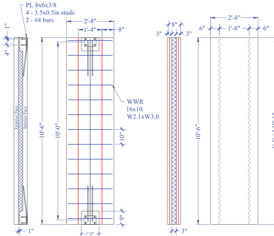
Figure 154. PCS 11 Panel Detail
