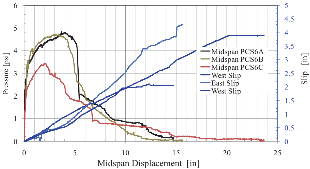
Figure 103. PCS6 Pressure–Displacement Response
