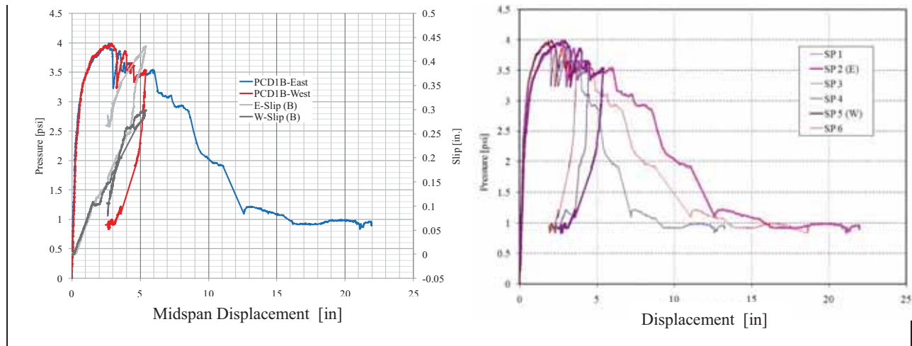
Figure 167. PCD1-B Response
