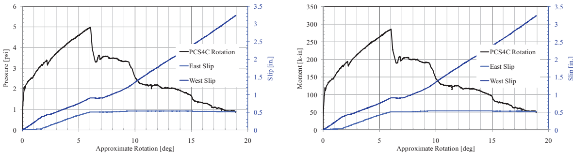
Figure 91. PCS4-C Response
