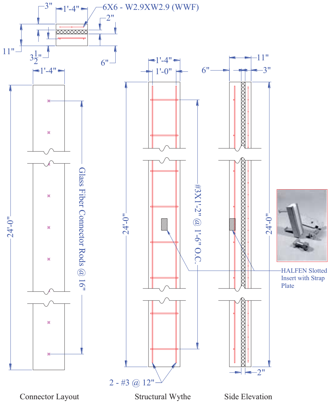
Figure 15. TCA Two-span Details TS3-A and B
