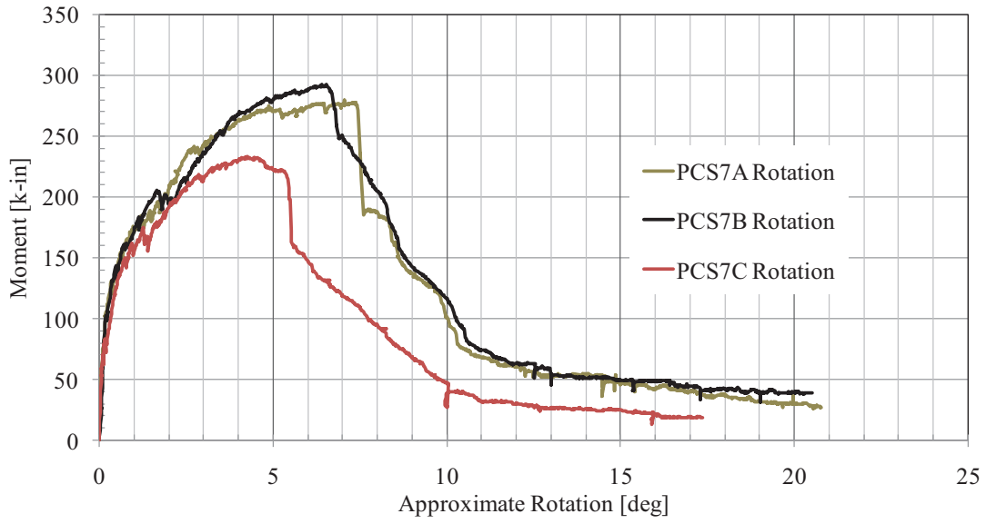
Figure 112. PCS7 Moment-Rotation Response
