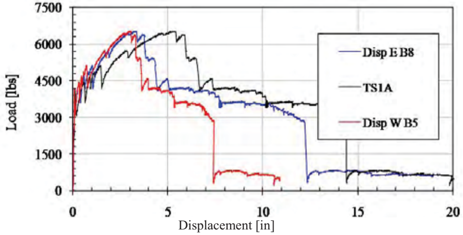
Figure 41. TS1-A Detail Results
