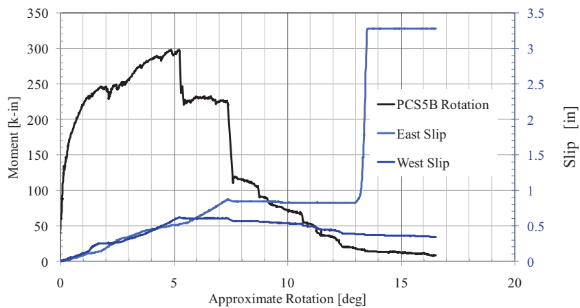
Figure 98. PCS5-B Response
