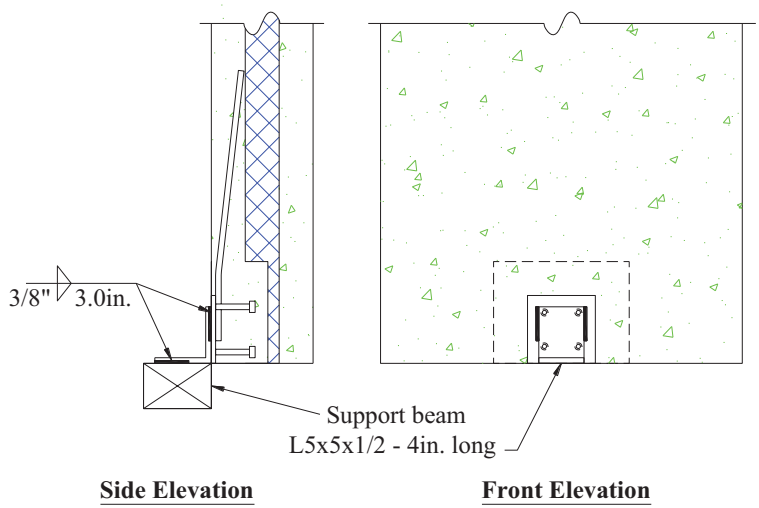
Figure 30. Embed to Support Connection Detail (PCS10 and 11)
