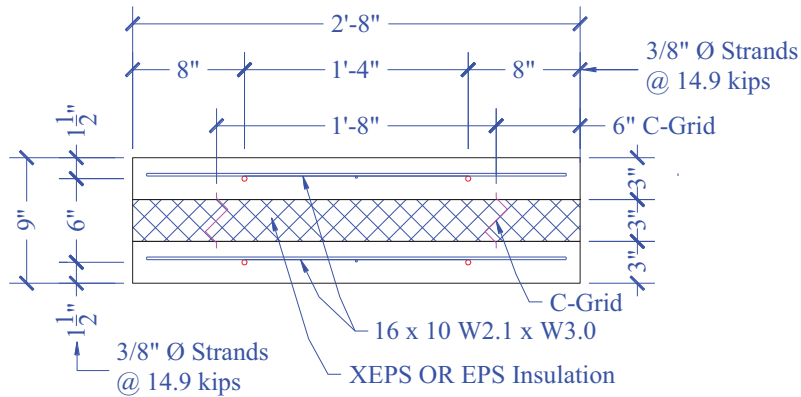
Figure 145. PCS10 Cross-Section Detail
