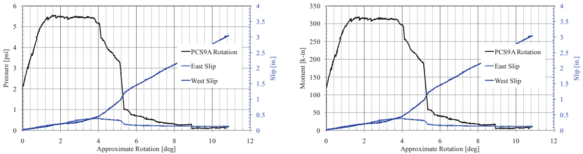
Figure 129. PCS9-A Response
