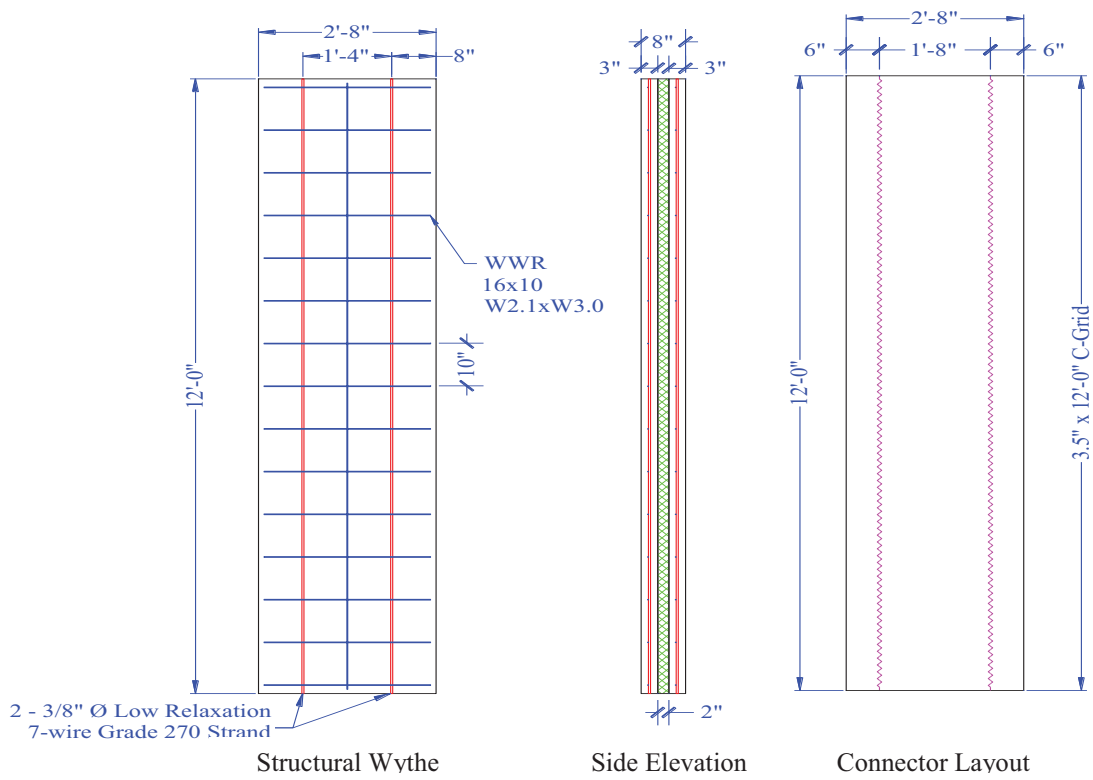
Figure 61. PCS2 Panel Detail
