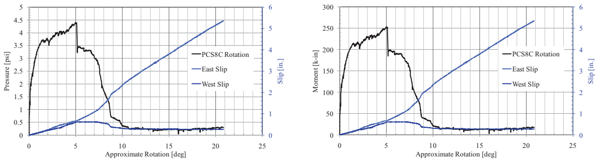
Figure 123. PCS8-C Response
