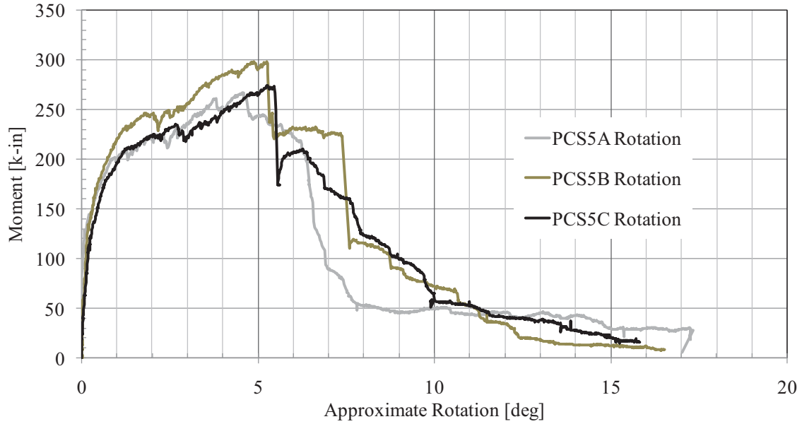
Figure 96. PCS5 Moment-Rotation Response
