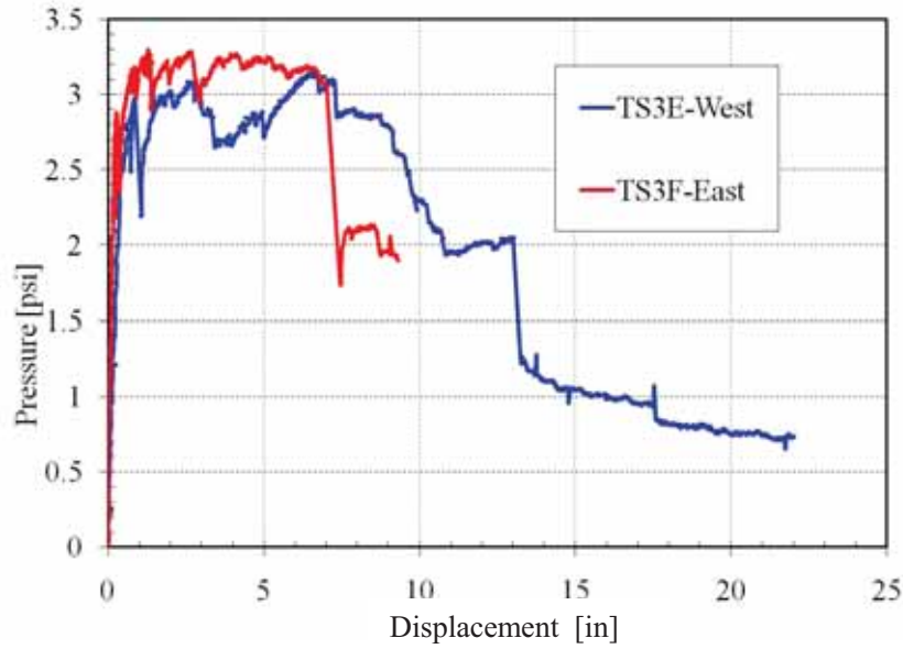
Figure 197. TS3-E, F Pressure-Displacement Response
