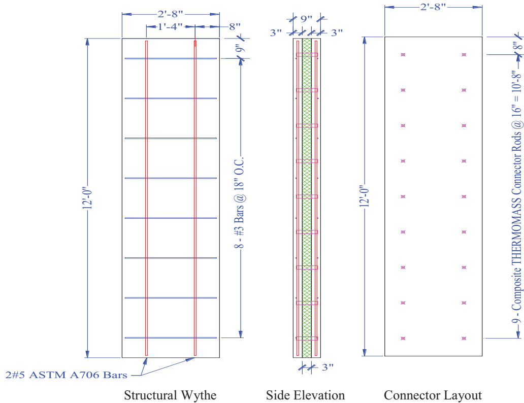
Figure 110. PCS7 Panel Detail
