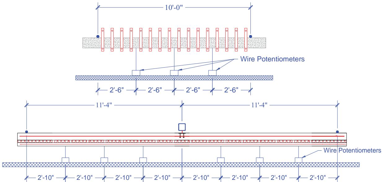
Figure 36. Displacement Instrumentation
