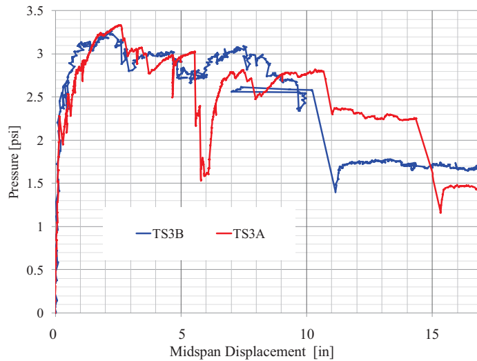
Figure 183. TS3-A, B Pressure-Displacement Response
