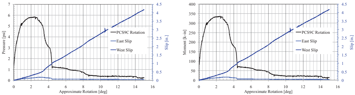
Figure 131. PCS9-C Response
