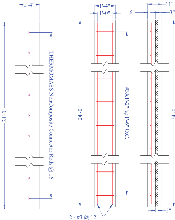
Figure 188. TS3-C, D Panel Detail
