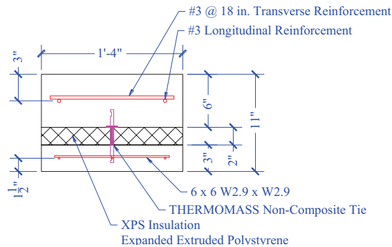
Figure 194. TS3-E, F Cross-Section Detail
