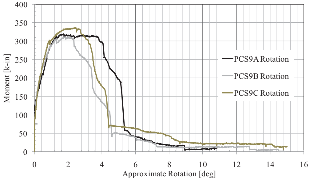
Figure 128. PCS9 Moment-Rotation Response
