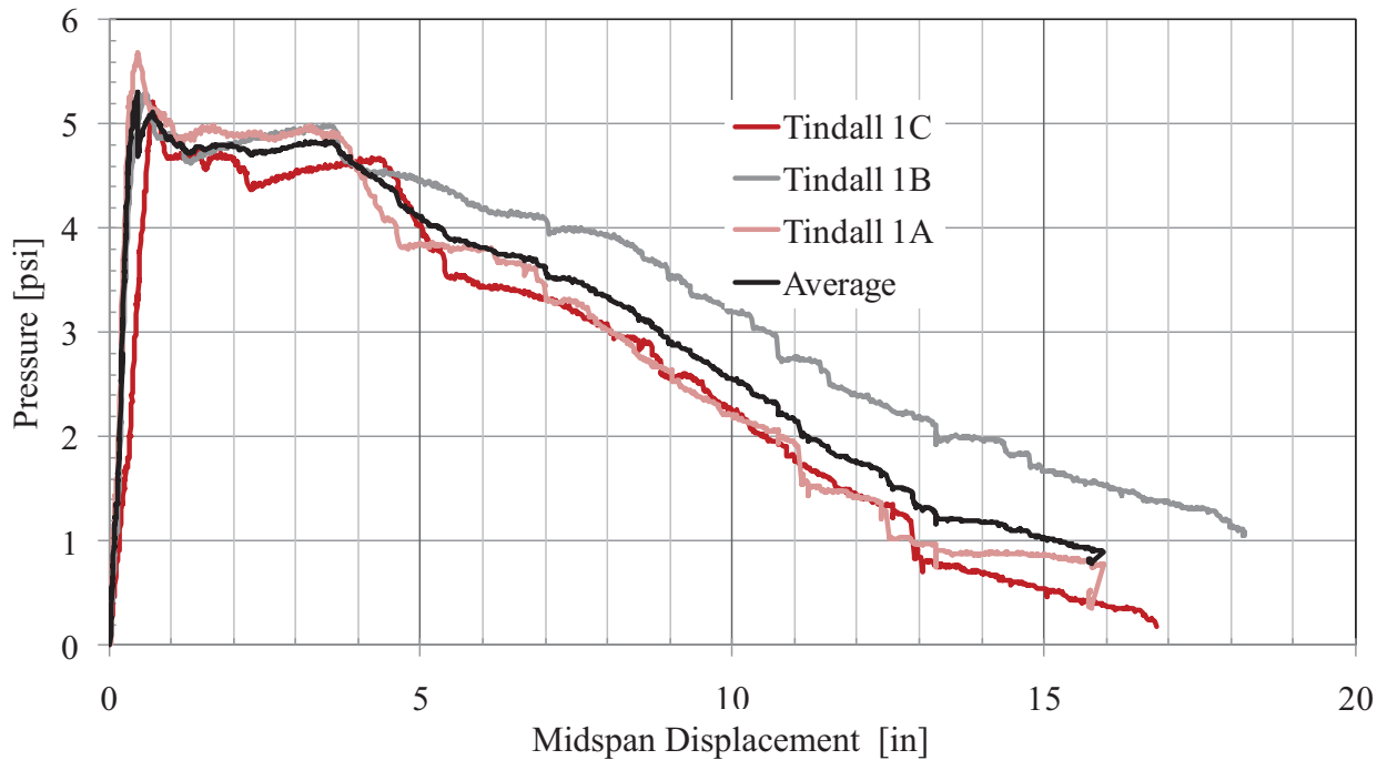
Figure 135. Tyn1 Pressure–Displacement Response
