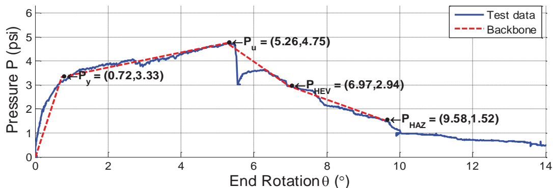
Figure 210. Backbone with Optimum Constants (1 psi = 6.9 kPa)
