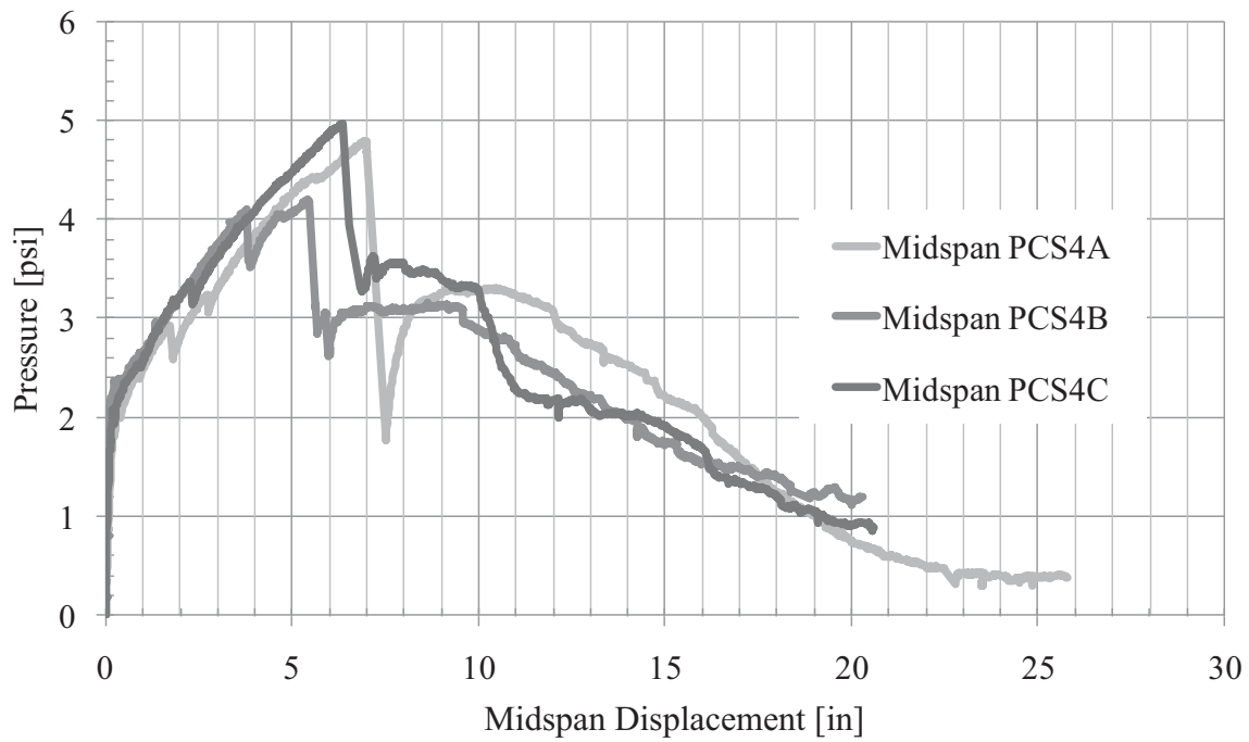
Figure 87. PCS4 Pressure-Displacement Response
