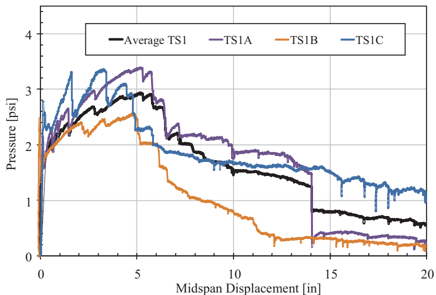
Figure 39. TS1 6-2-3 Pressure—Midspan Displacement
