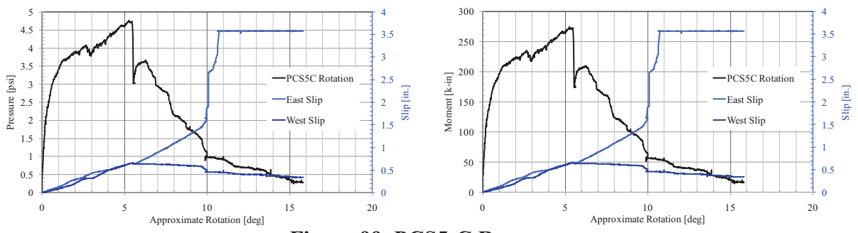
Figure 99. PCS5-C Response
