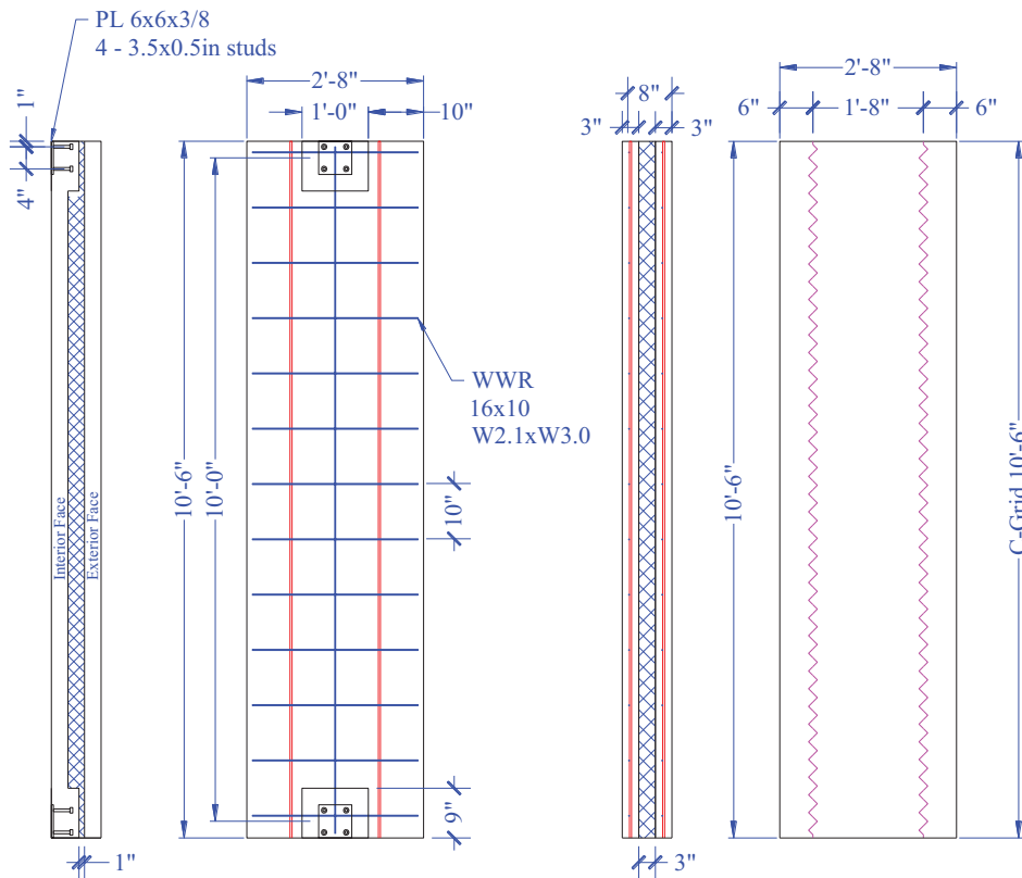
Figure 146. PCS10 Panel Detail
