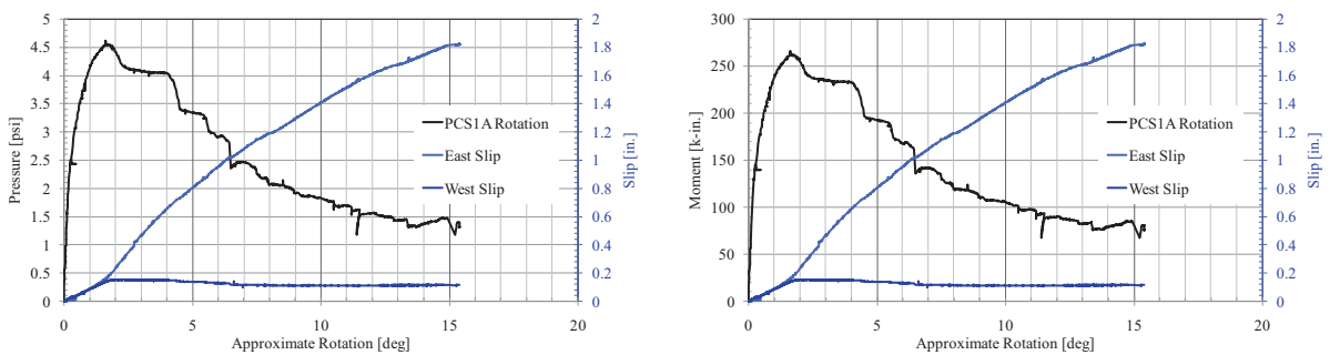
Figure 56. PCS1-A Response
