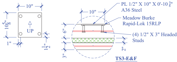
Figure 196. TS3-E, F Connection Detail
