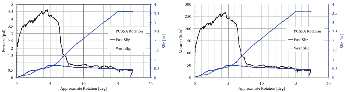
Figure 97. PCS5-A Response
