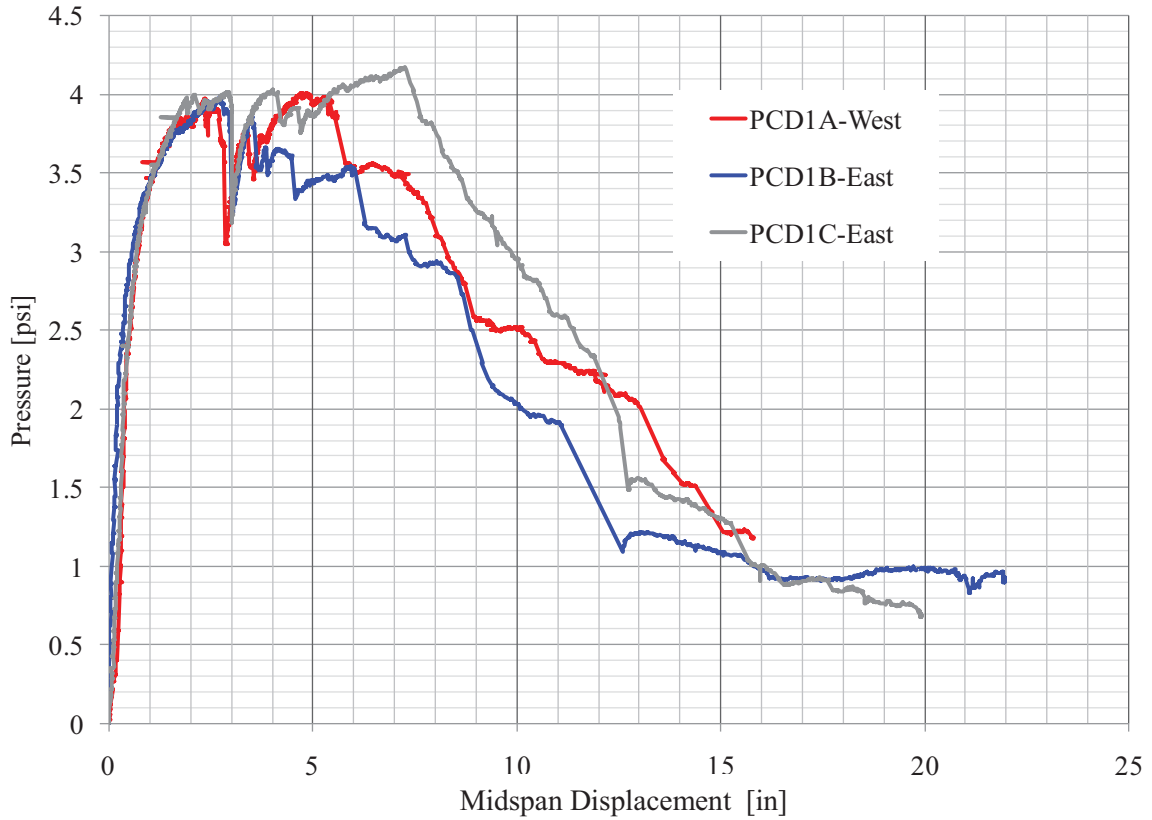
Figure 164. PCD1 Pressure–Displacement Response
