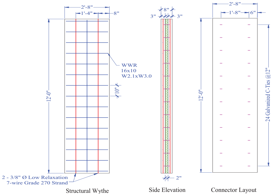
Figure 53. PCS1 Panel Detail
