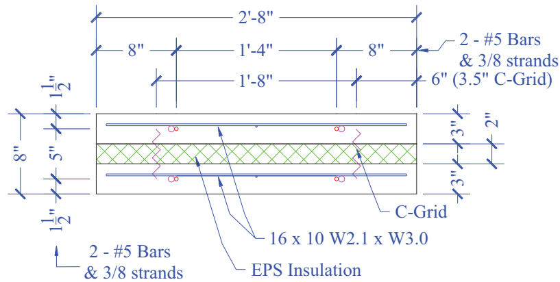
Figure 76. PCS3 (Type 2) Cross-Section Detail
