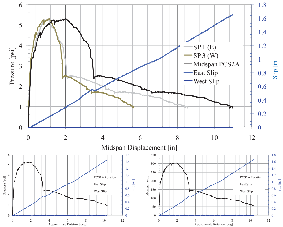
Figure 64. PCS2-A Response
