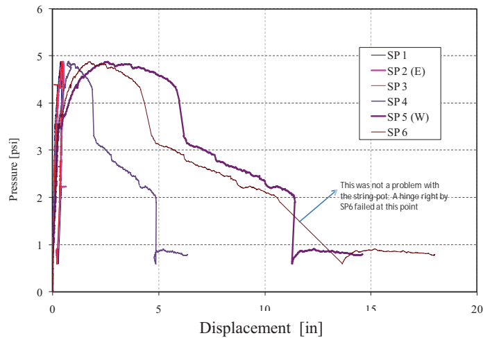
Figure 177. PCD2-B Response
