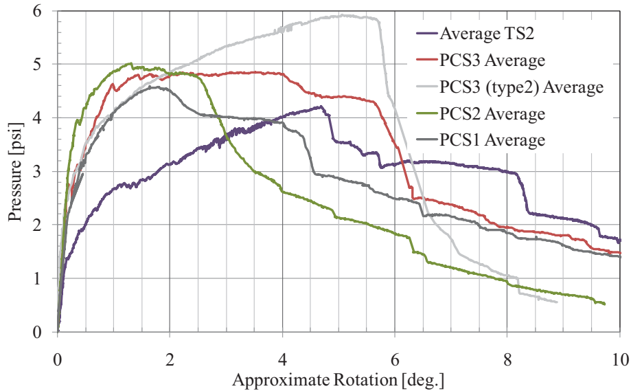
Figure 202. Average Single-span Response 3-2-3 Panels
