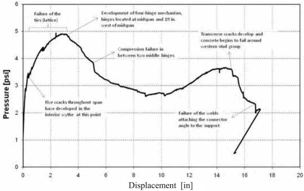
Figure 157. PCS11-A Response
