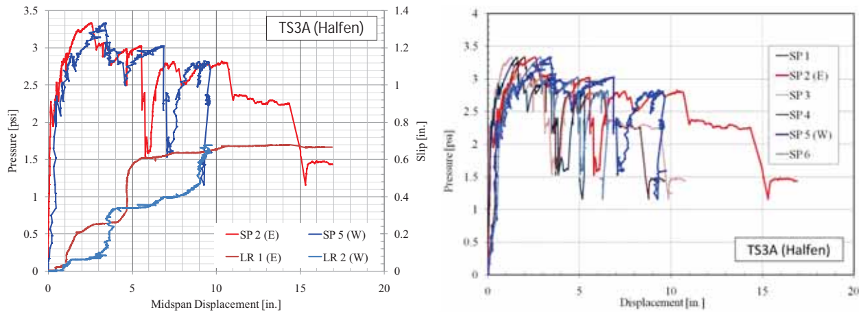
Figure 184. TS3-A Response
