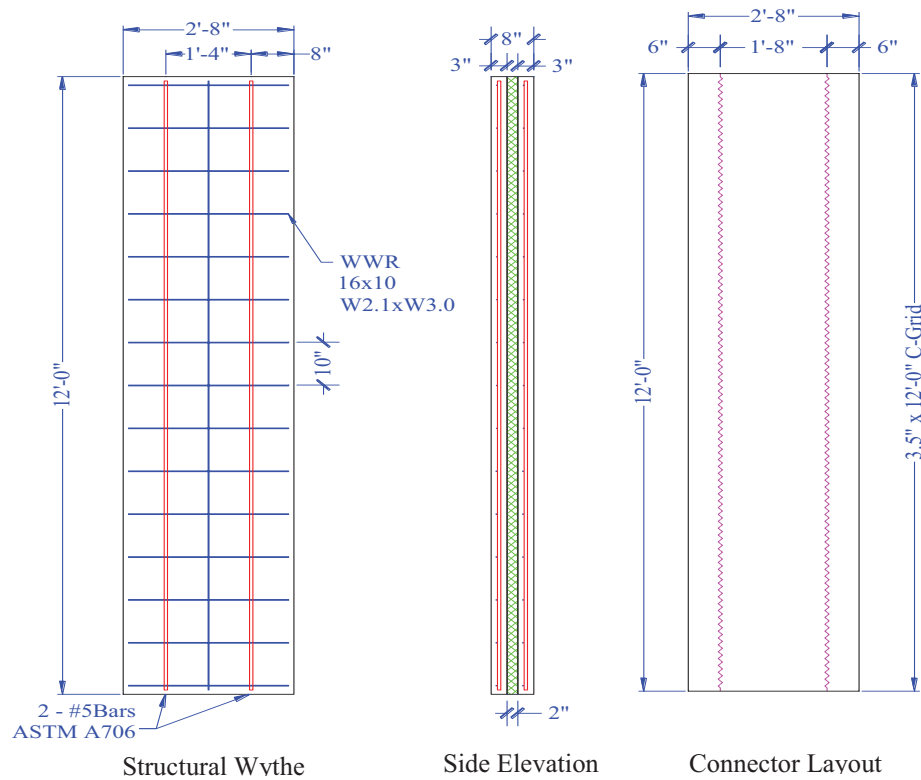
Figure 69. PCS3 Panel Detail
