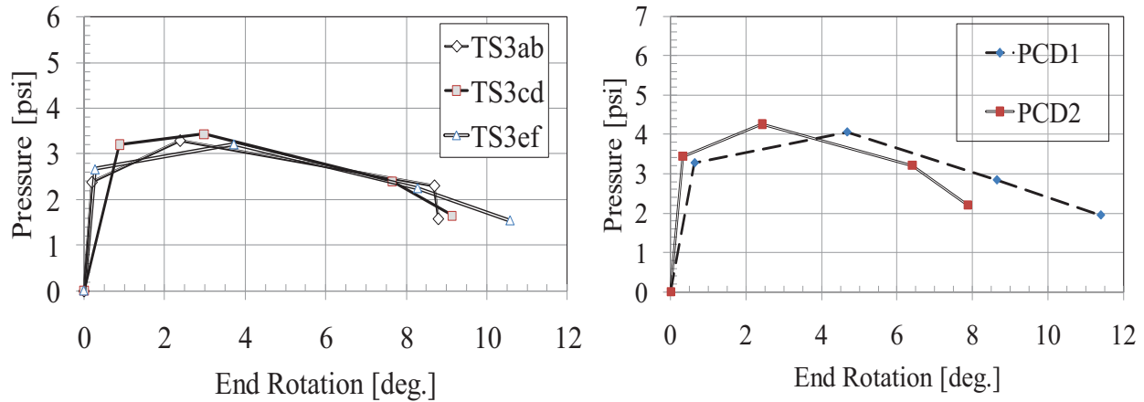
Figure 215. Backbone Curves
