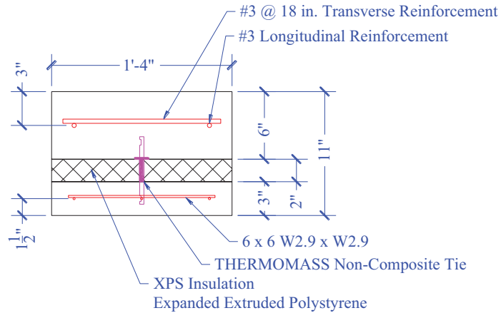
Figure 187. TS3-C, D Cross-Section Detail
