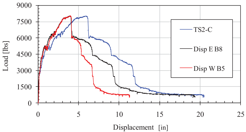
Figure 50. TS2-C Detail Results
