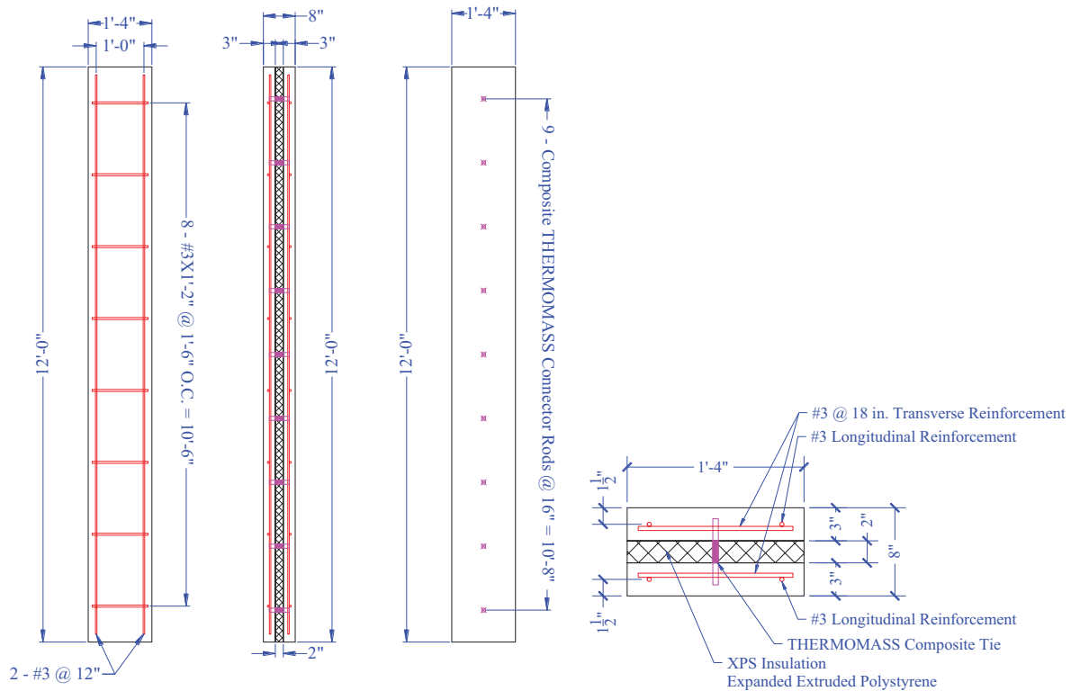
Figure 45. TS2 Reinforcement Details
