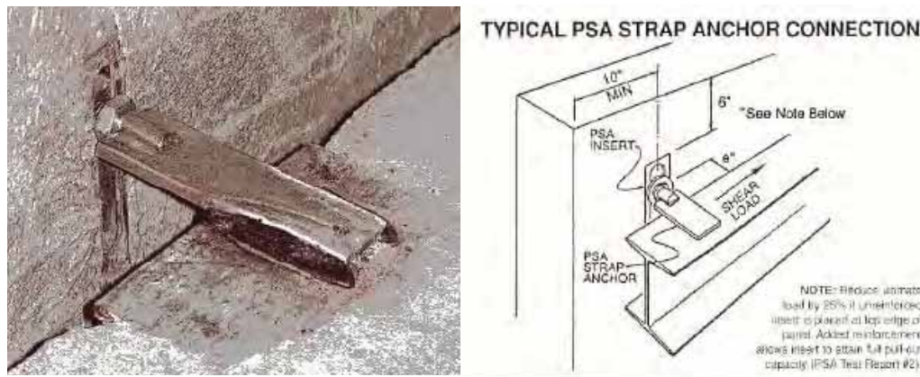
Figure 22. JVI PSA Insert
