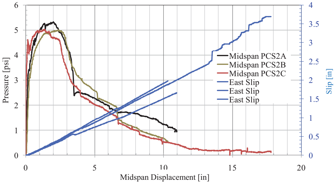
Figure 62. PCS2 Pressure-Displacement Response
