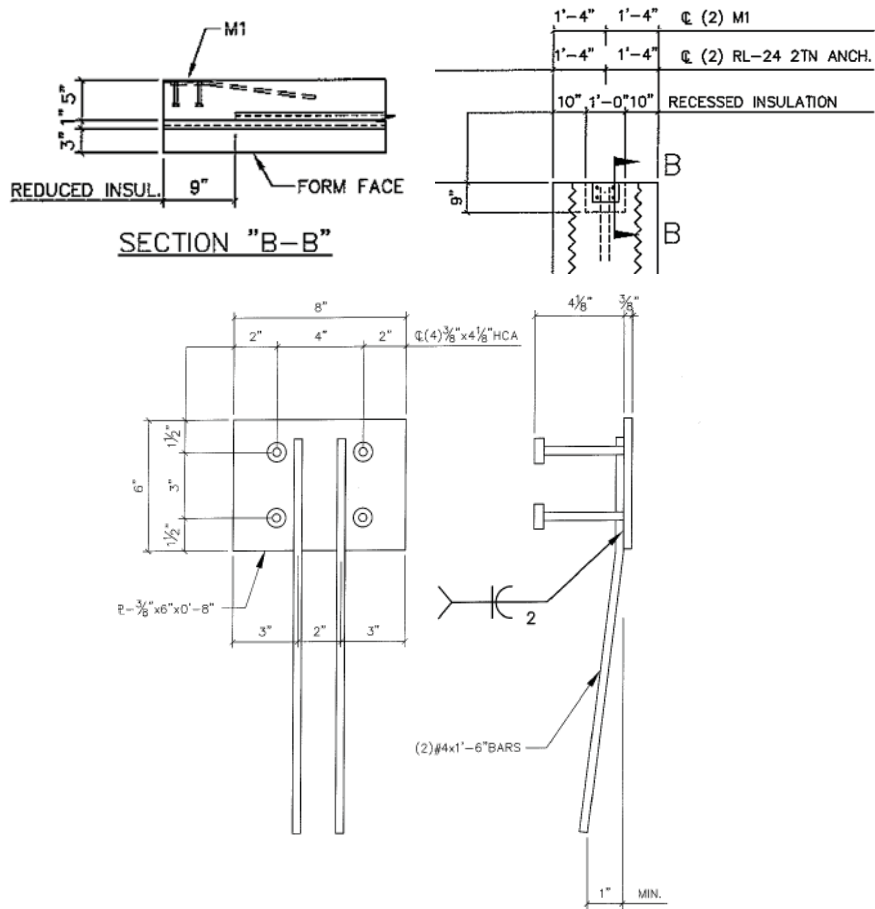
Figure 29. PCS11 Connection Details
