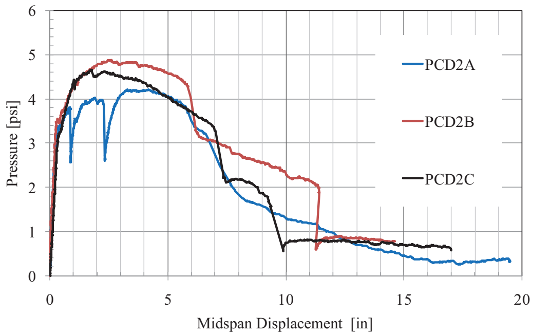
Figure 175. PCD2 Pressure–Displacement Response
