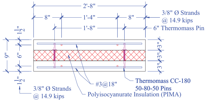
Figure 117. PCS8 Cross-Section Detail
