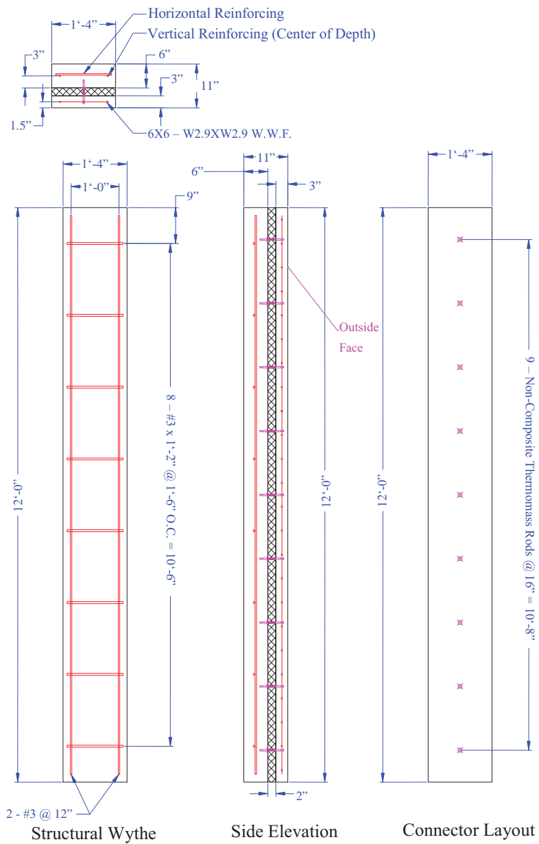
Figure 8. TCA Non-composite 6-2-3 Single-span Static Specimen TS1 Details
