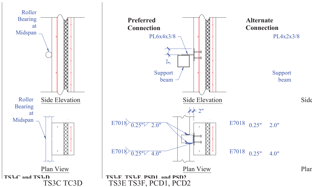
Figure 24. Connection Details
