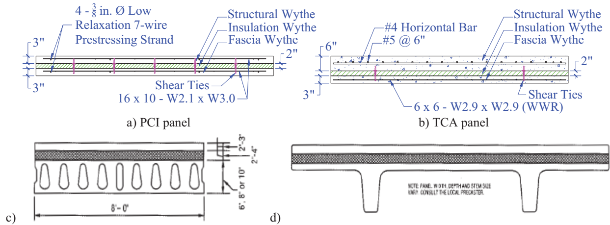
Figure 4. TCA and PCI Wall Sections (c and d [PCI 1997])
