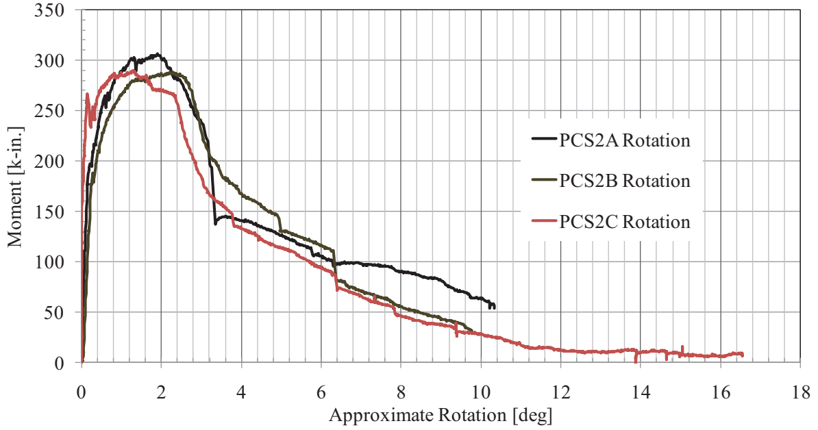
Figure 63. PCS2 Moment-Rotation Response
