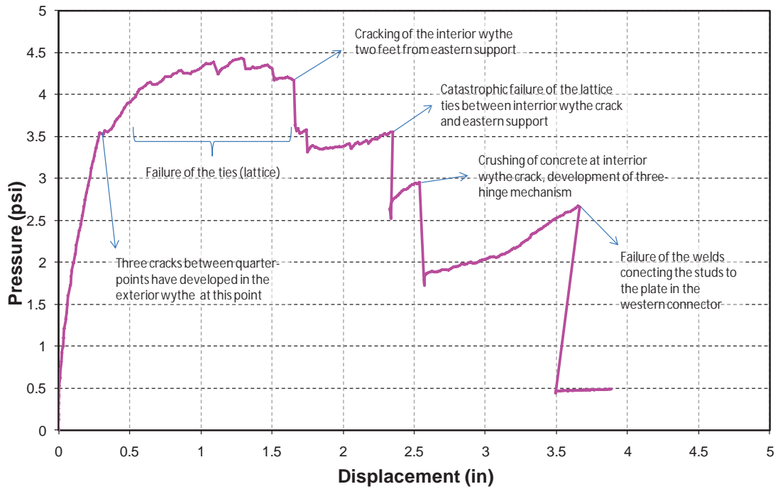
Figure 150. PCS10-B Rebound Response
