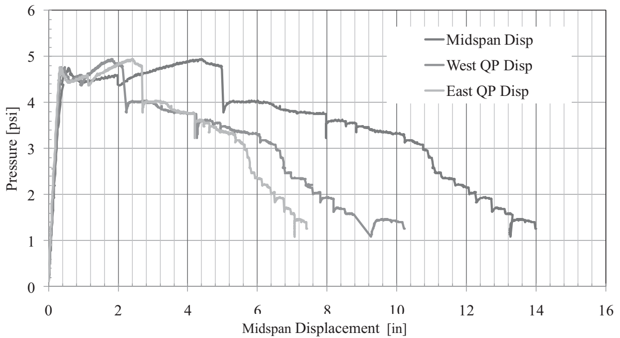
Figure 144. Tyn2-C Response
