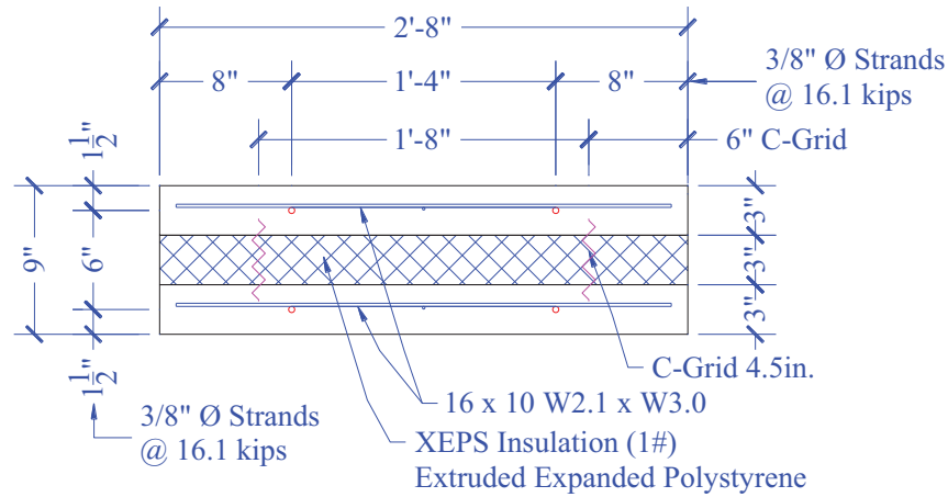
Figure 101. PCS6 Cross-Section Detail
