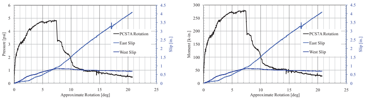
Figure 113. PCS7-A Response
