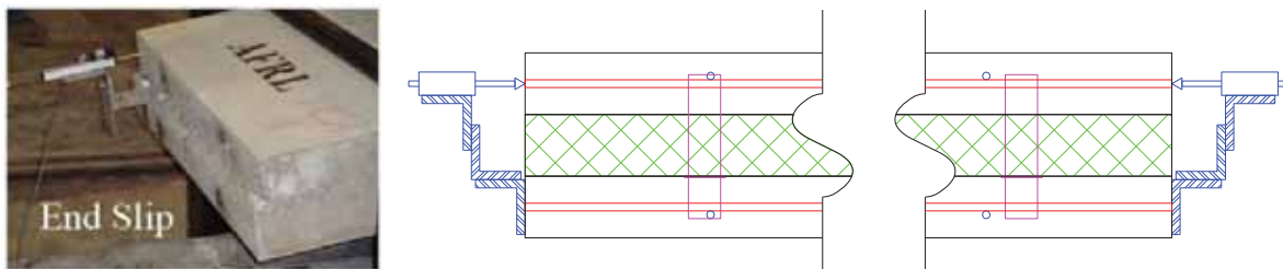
Figure 37. End Shear Instrumentation
