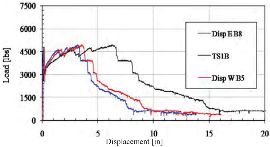
Figure 42. TS1-B Detail Results
