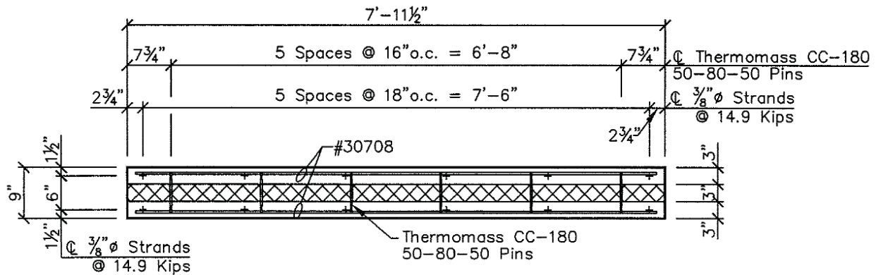
Figure 11. Coreslab PCI Prototype Wall Panel Design
