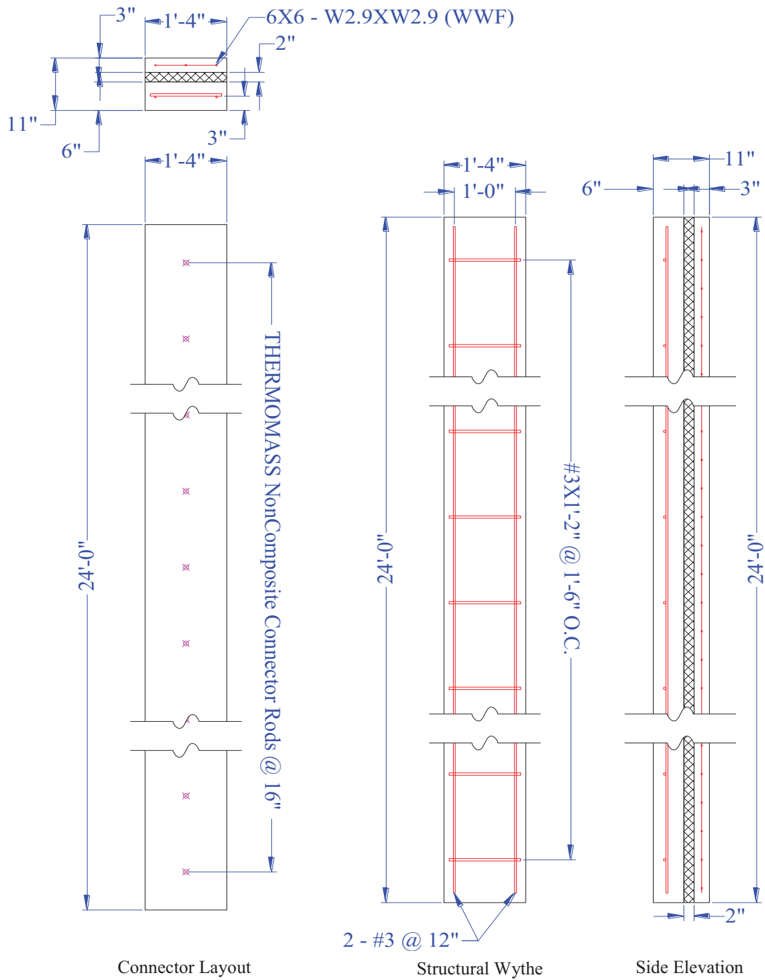
Figure 16. TCA Two-span Details TS3-C and D
