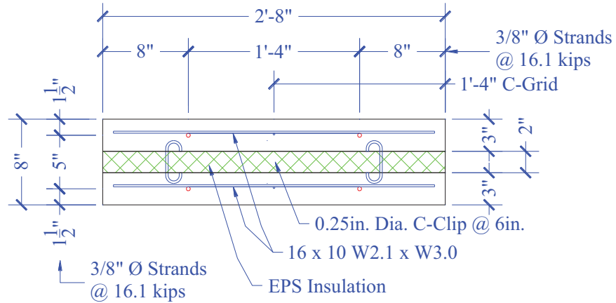
Figure 52. PCS1 Cross-Section Detail
