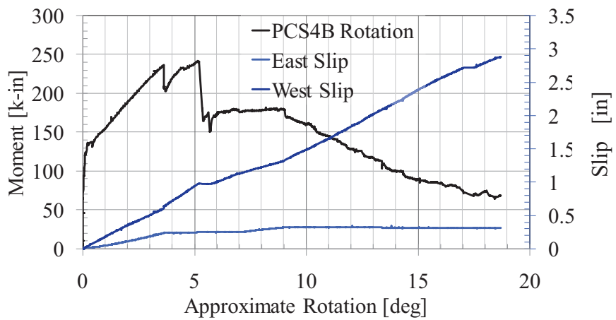
Figure 90. PCS4-B Response
