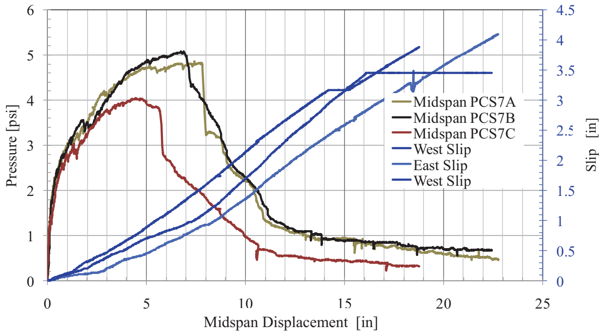
Figure 111. PCS7 Pressure–Displacement Response
