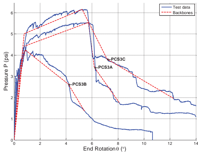
Figure 208. Pressure–Rotation Characterization (1 psi = 6.9kPa)
