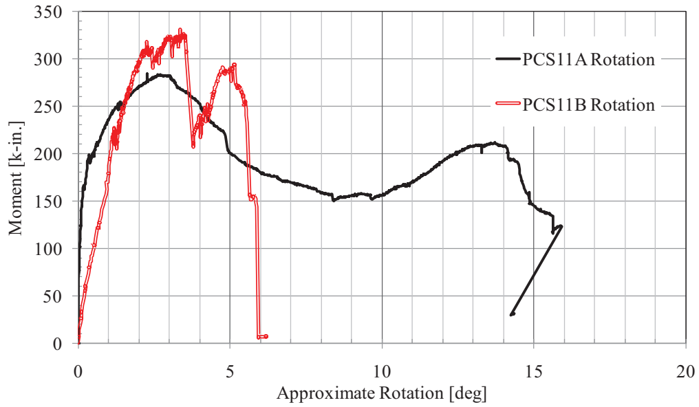
Figure 156. PCS11 Moment-Rotation Response
