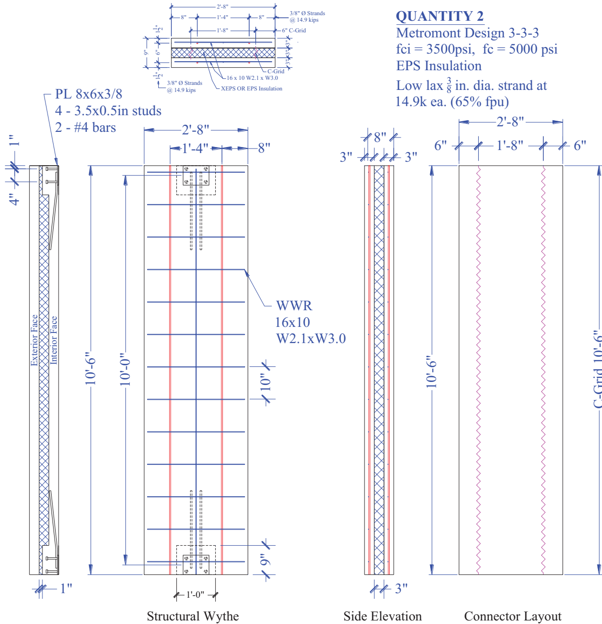
Figure 26. Specimen PCS11—Base Connection
