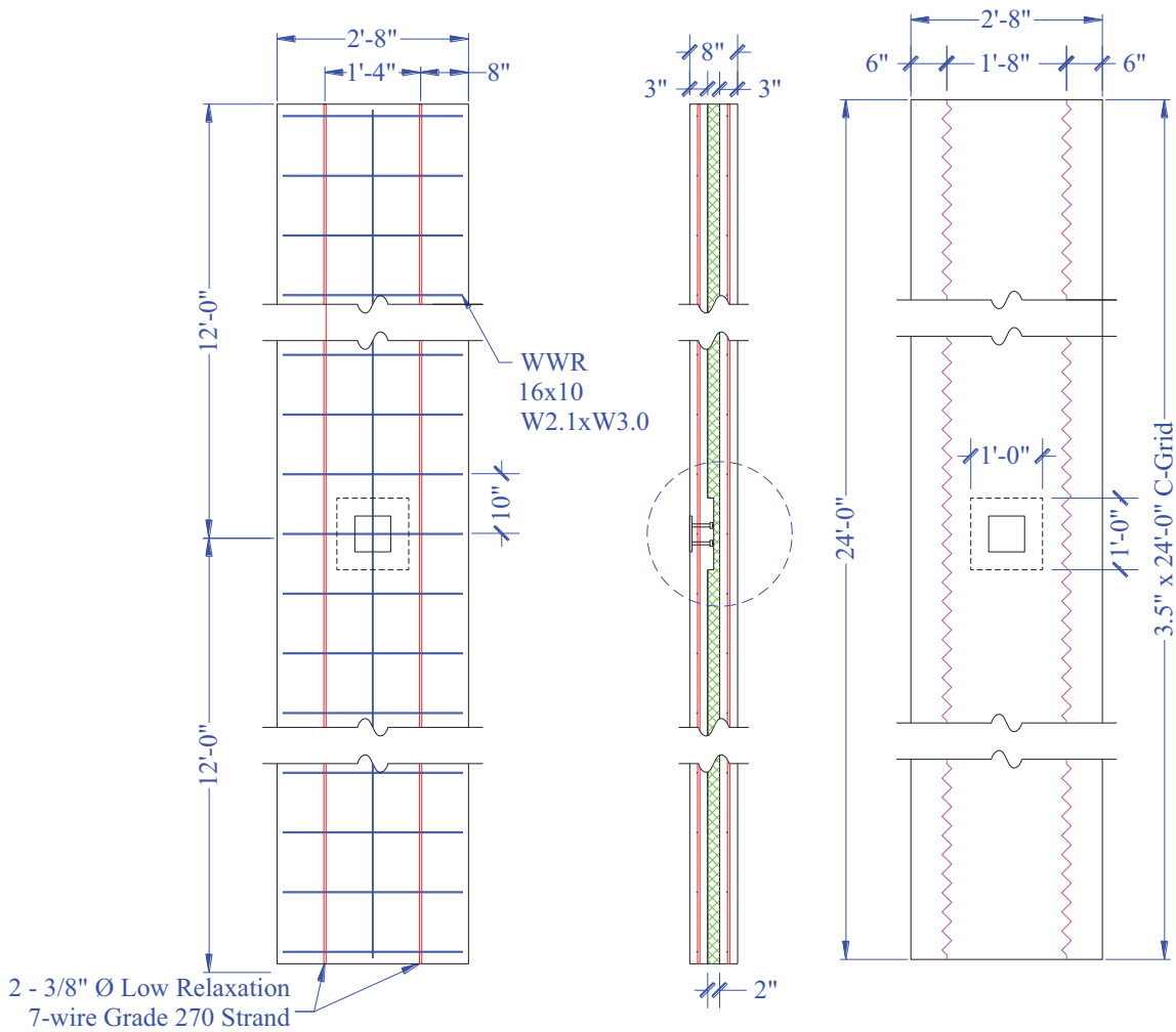
Figure 173. PCD2 Panel Detail
