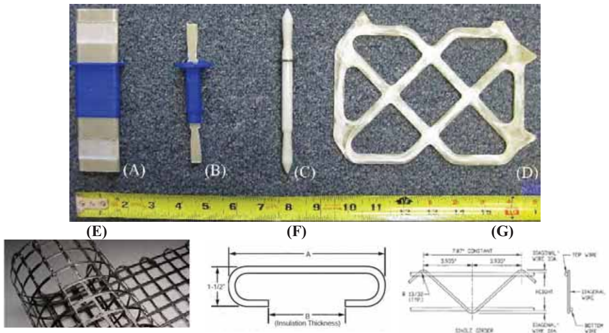
Figure 5. Shear Ties Samples
