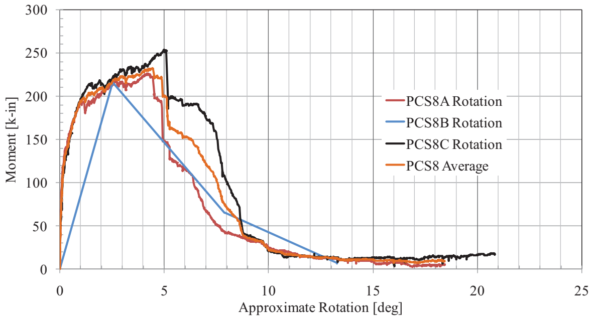
Figure 120. PCS8 Moment-Rotation Response
