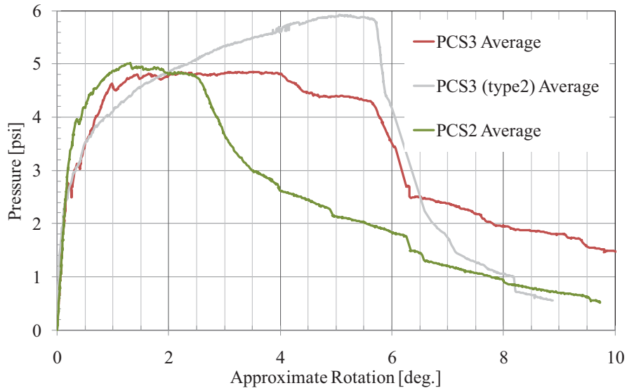
Figure 206. Prestressed versus Non-PS Reinforcement
