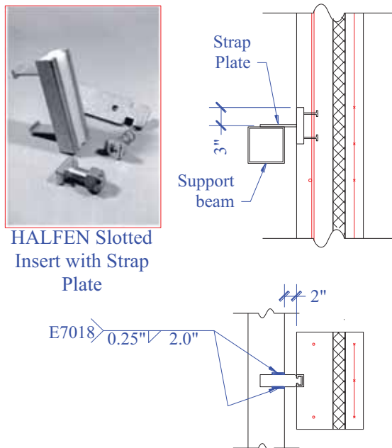
Figure 182. TS3-A, B Connection Detail
