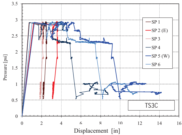
Figure 191. TS3-C Response
