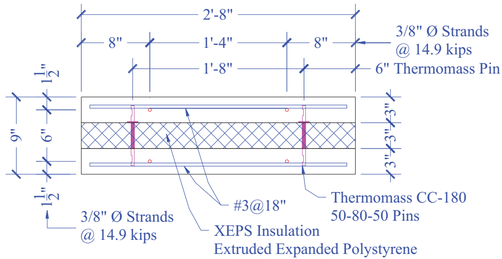
Figure 93. PCS5 Cross-Section Detail
