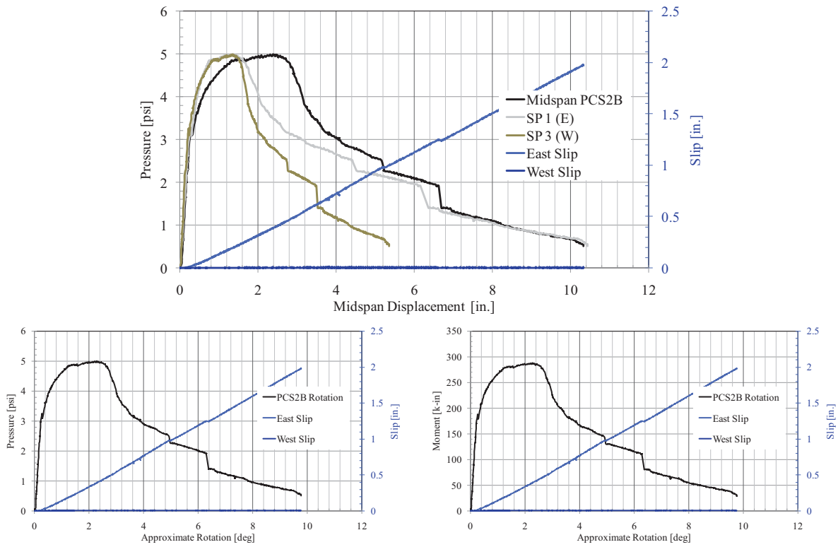
Figure 65. PCS2-B Pressure-Displacement Response
