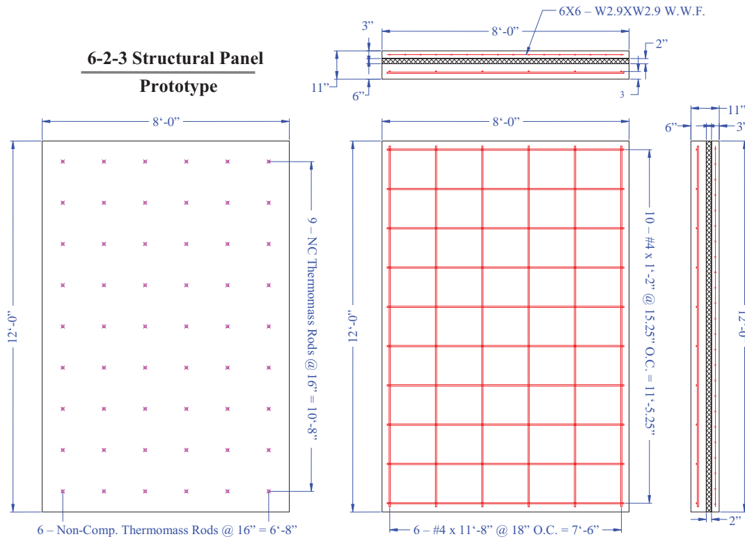
Figure 7. Prototype TCA 6-2-3 Wall
