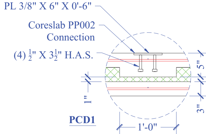
Figure 163. Coreslab Two-span Panel PCD1 Midspan Connection
