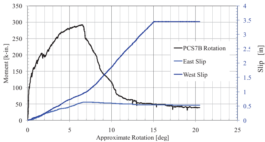
Figure 114. PCS7-B Response
