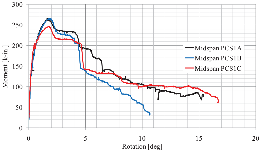
Figure 55. PCS1 Moment-Rotation Response
