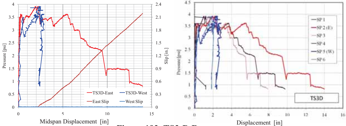
Figure 192. TS3-D Response
