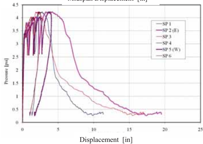
Figure 176. PCD2-A Response
