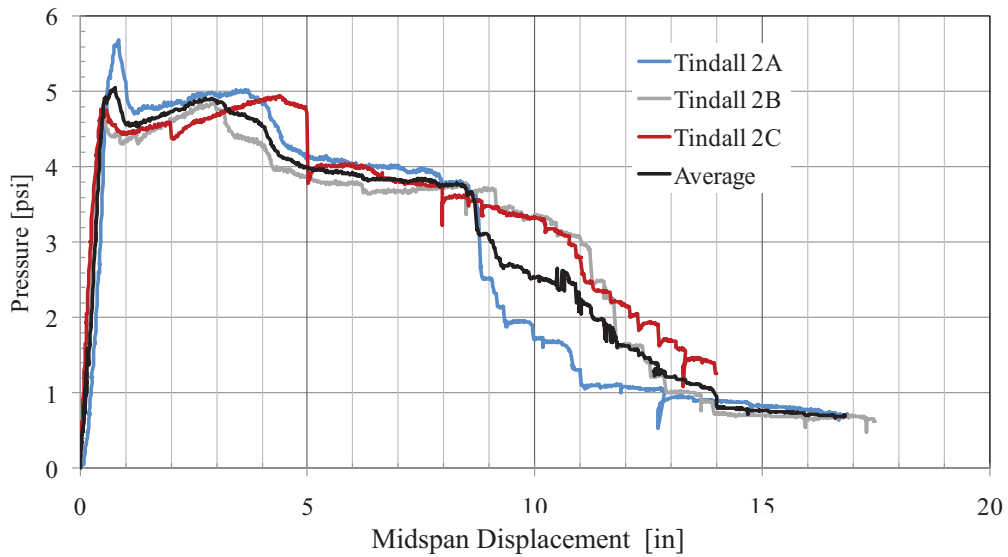
Figure 141. Tyn2 Pressure-Displacement Response
