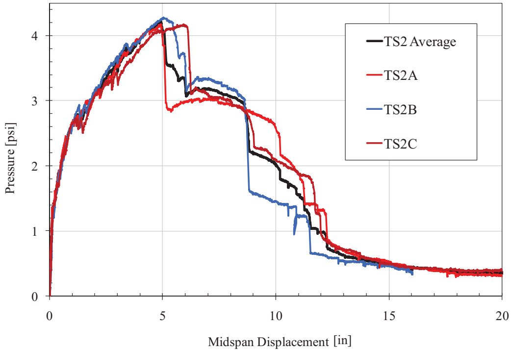
Figure 46. 3-2-3 Pressure—Midspan Displacement
