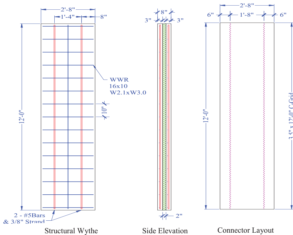
Figure 77. PCS3 (Type 2) Panel Detail
