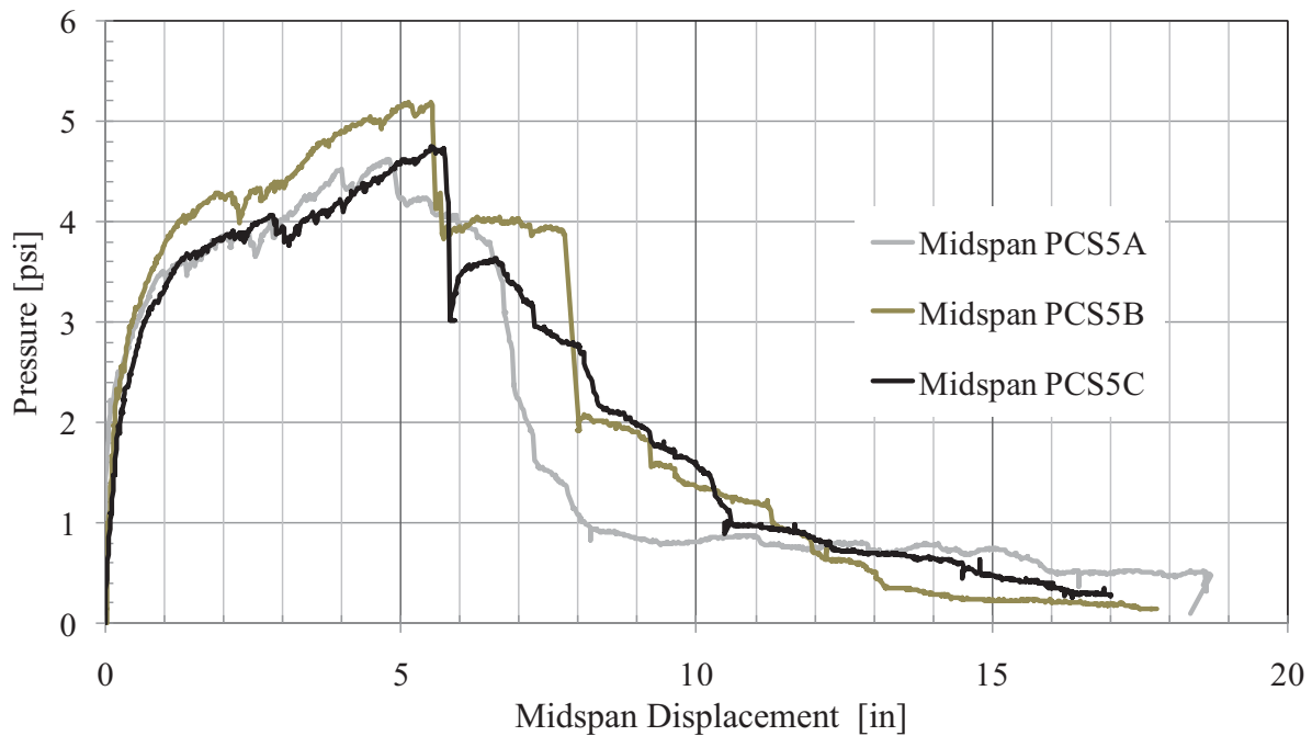
Figure 95. PCS5 Pressure–Displacement Response
