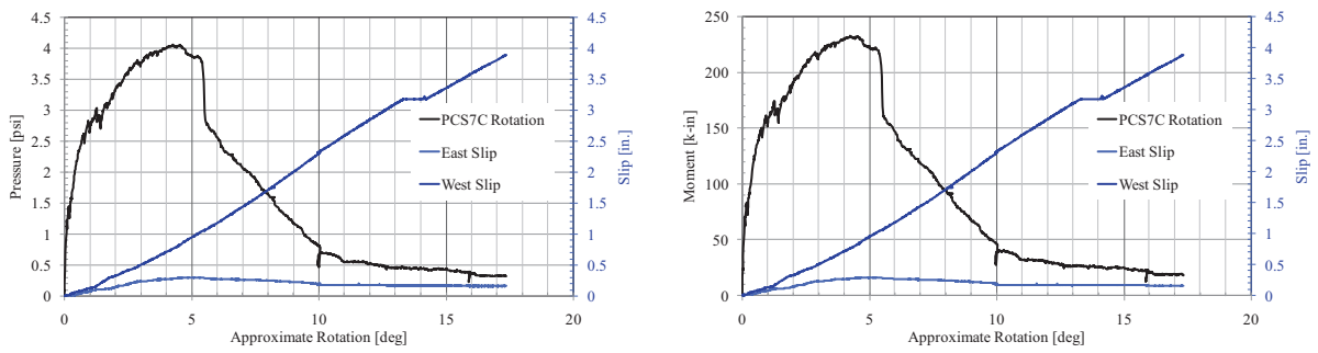
Figure 115. PCS7-C Response
