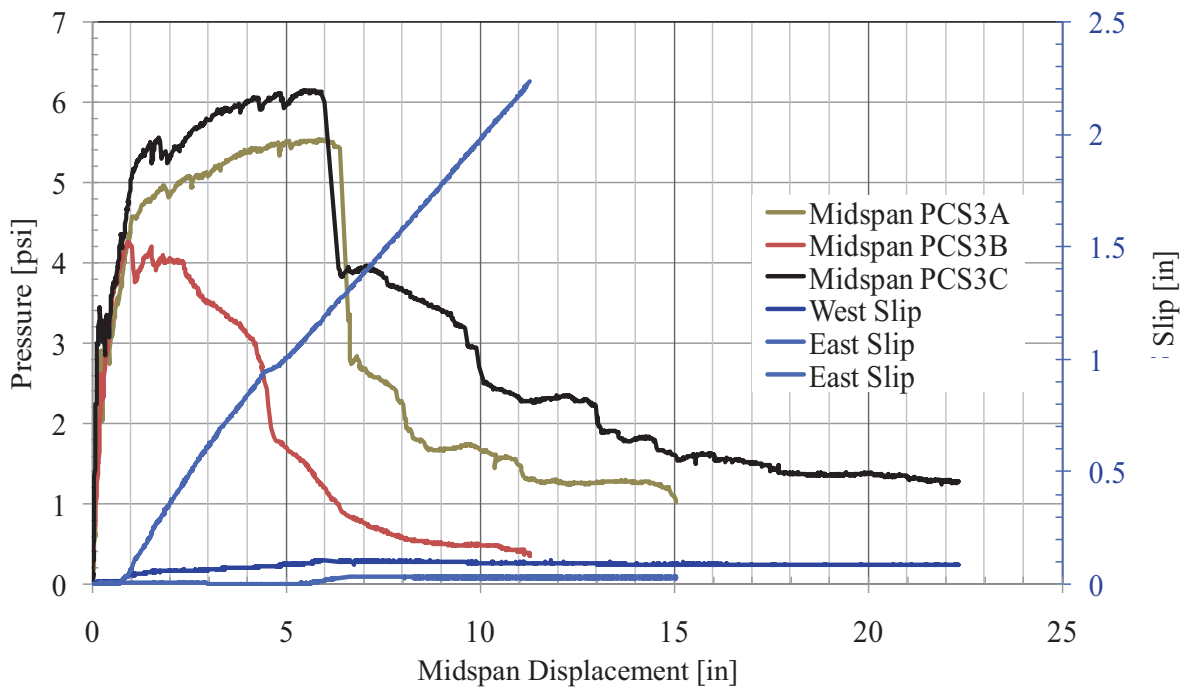
Figure 70. PCS3 Pressure-Displacement Response
