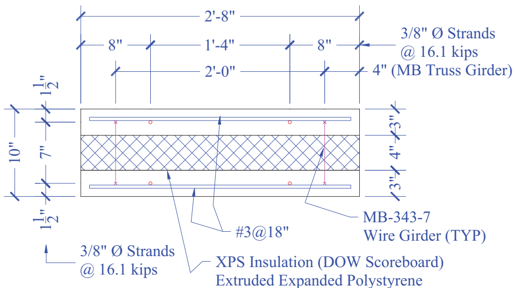
Figure 139. Tyn2 Cross-Section Detail
