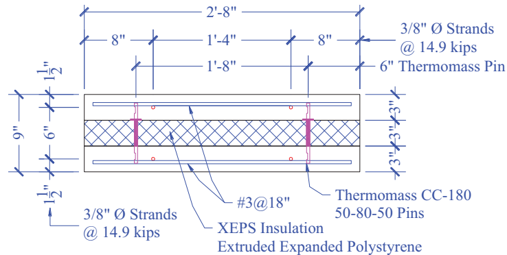
Figure 161. PCD1 Cross-Section Detail
