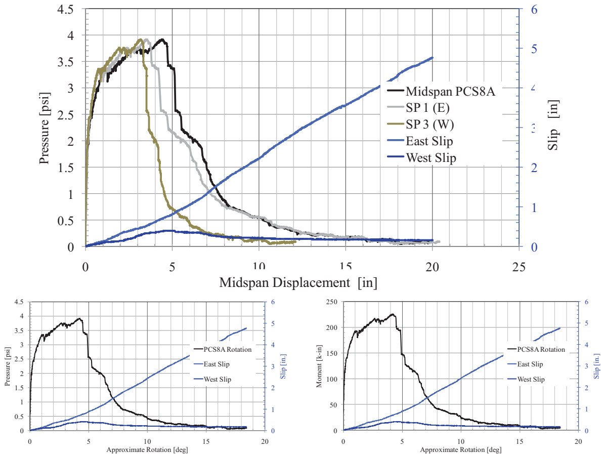
Figure 121. PCS8-A Response
