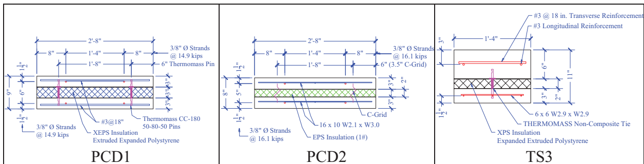
Figure 213. Two-span Sections
