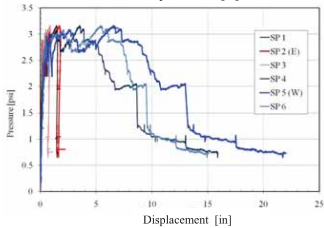
Figure 198. TS3-E Inbound Response
