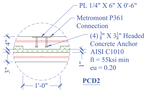
Figure 174. PCD2 Midspan Connection Detail
