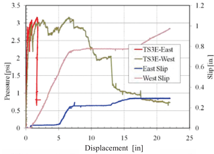
Figure 197. TS3-E, F Pressure-Displacement Response
