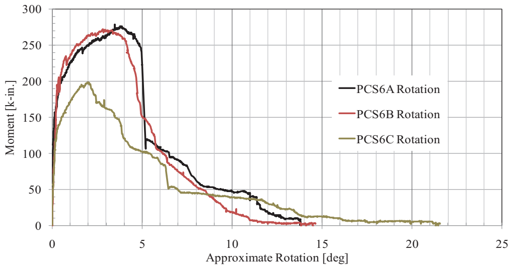
Figure 104. PCS6 Moment–Rotation Response
