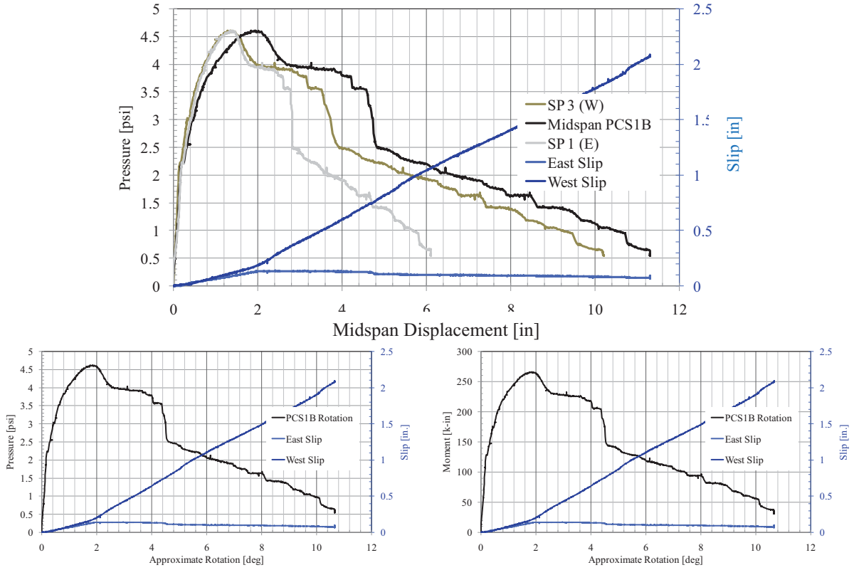
Figure 57. PCS1-B Response
