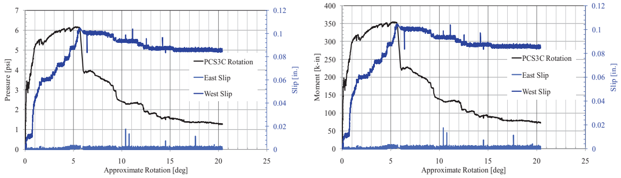
Figure 74. PCS3-C Response
