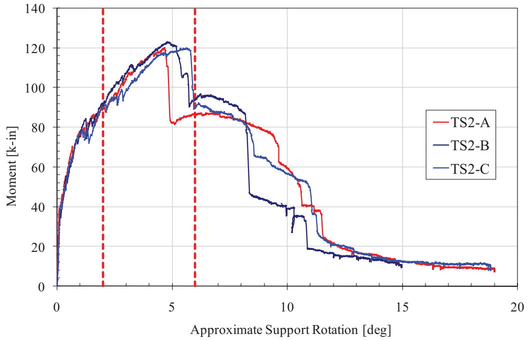
Figure 47. TS2 3-2-3 Moment Rotation at Midspan
