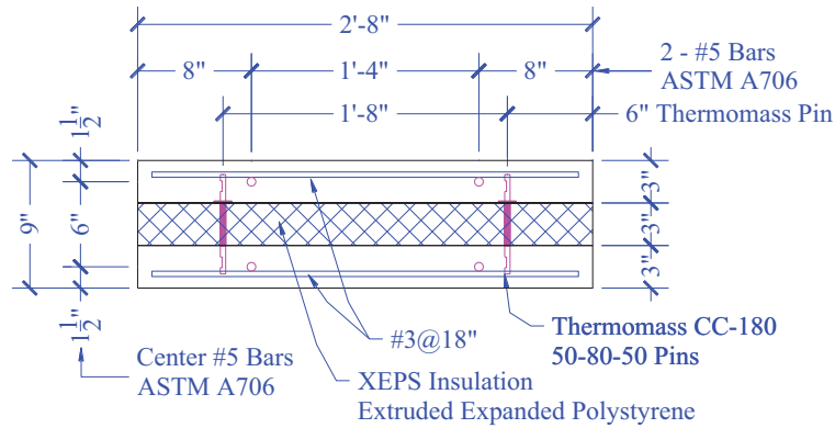
Figure 109. PCS7 Cross-Section Detail
