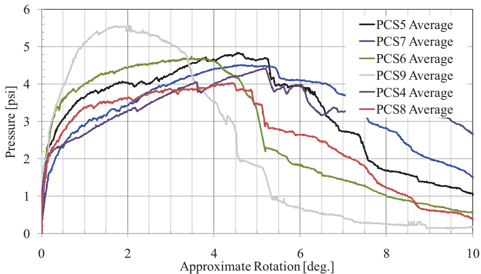
Figure 203. Average Single-span Response 3-2-3 Panels
