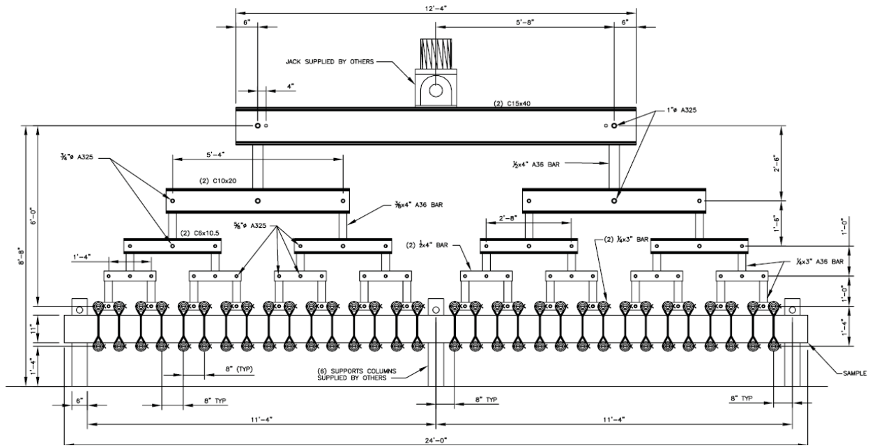
Figure 33. Two-span Loading Tree
