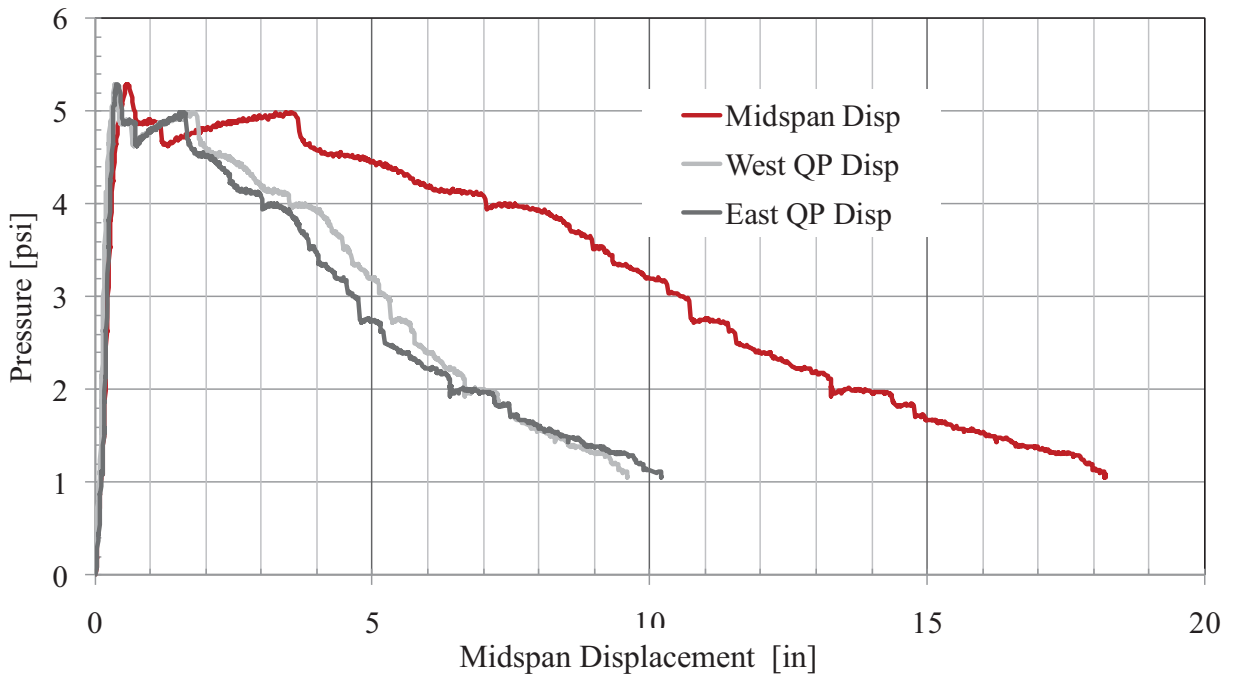
Figure 137. Tyn1-B Response
