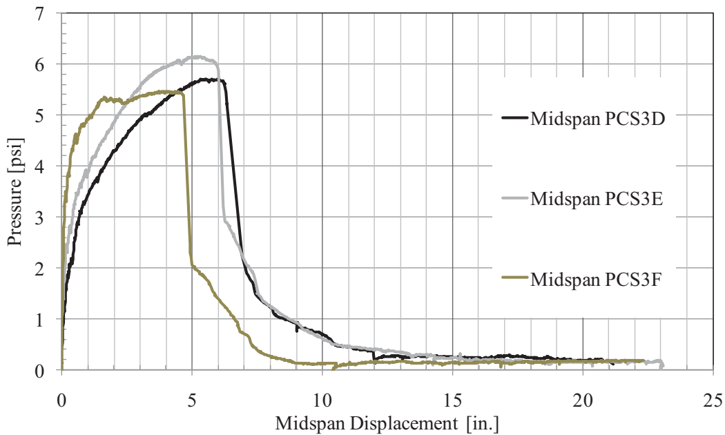
Figure 78. PCS3 (Type 2) Pressure–Displacement Response
