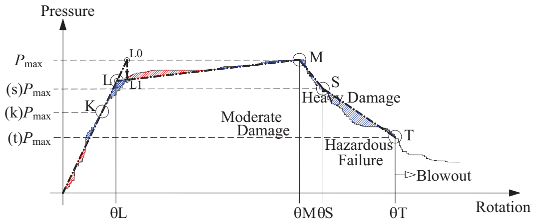
Figure 209. Backbone Development
