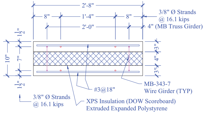
Figure 133. Tyn1 Cross-Section Detail
