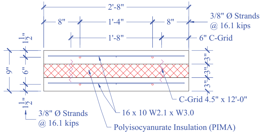
Figure 125. PCS9 Cross-Section Detail
