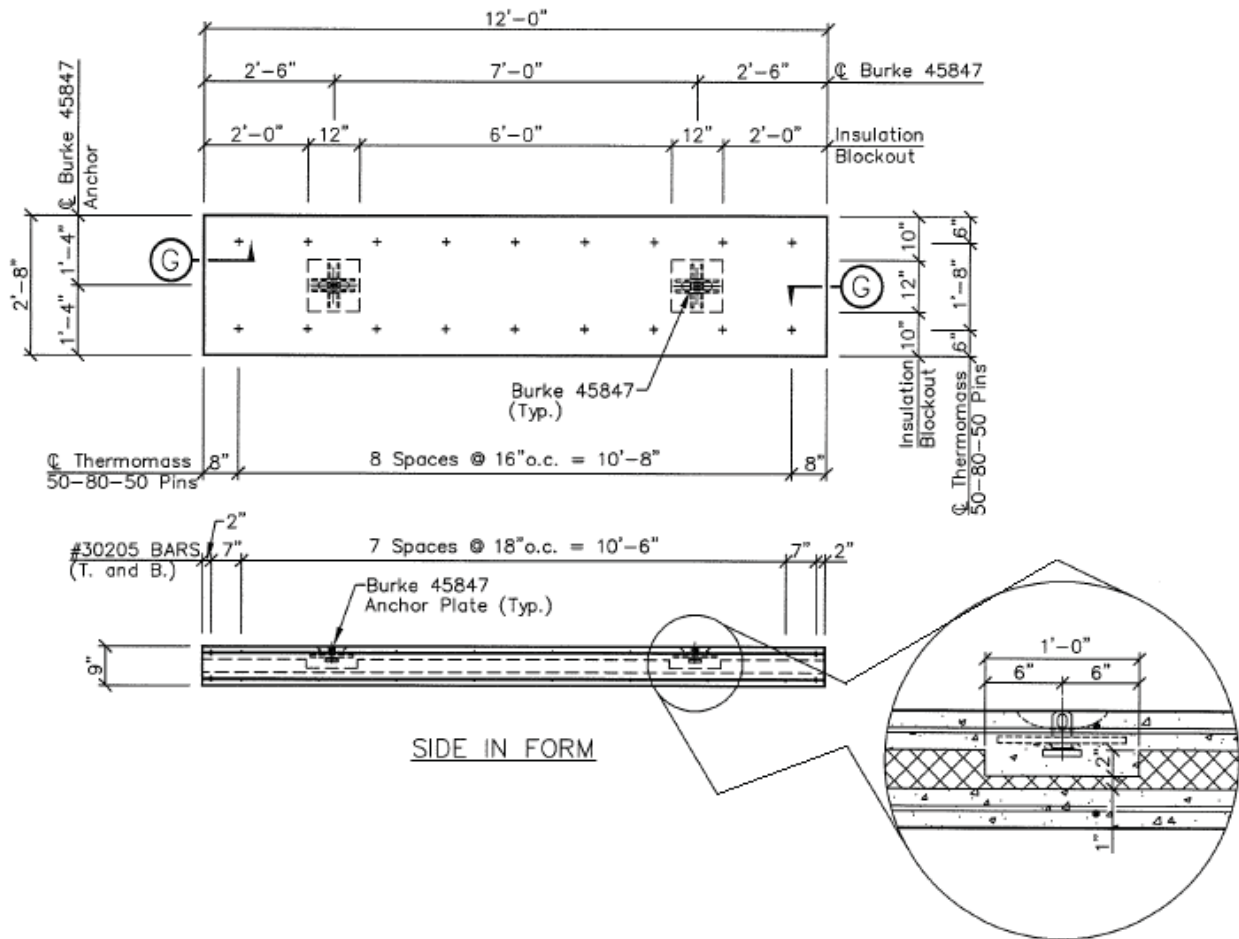
Figure 94. PCS5 Panel Detail
