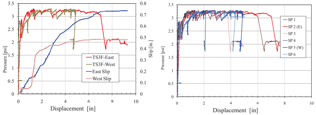
Figure 199. TS3-F Rebound Response
