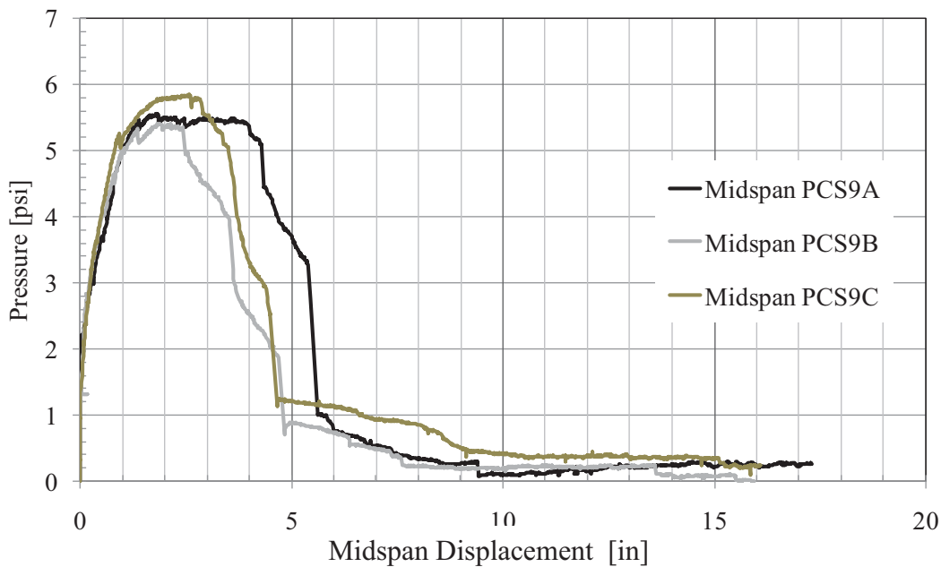
Figure 127. PCS9 Pressure–Displacement Response
