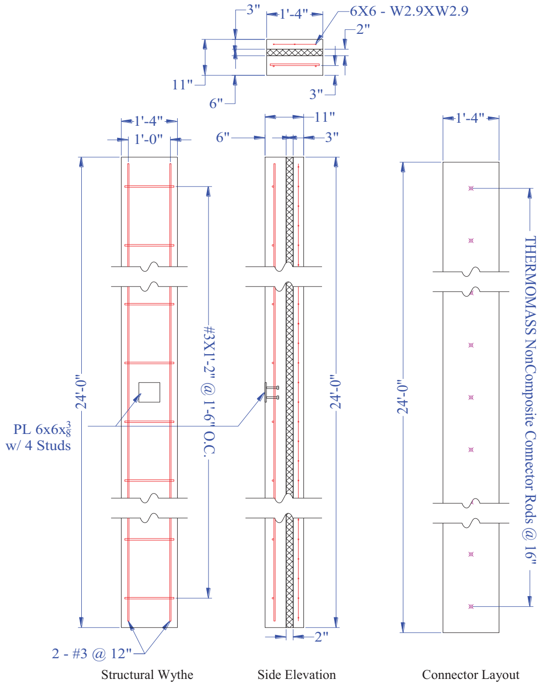
Figure 17. TCA Two-span Details TS3-E and F
