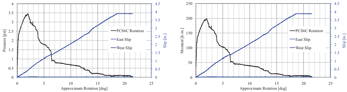
Figure 107. PCS6-C Response
