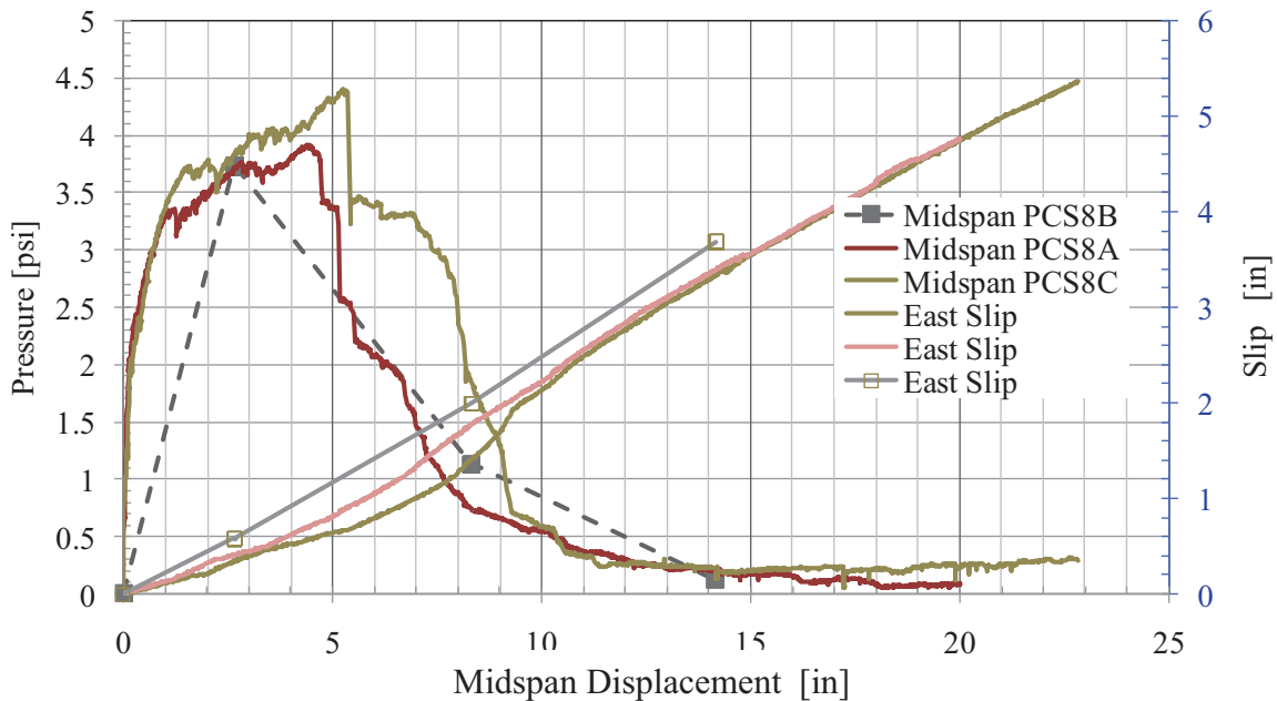
Figure 119. PCS8 Pressure–Displacement Response
