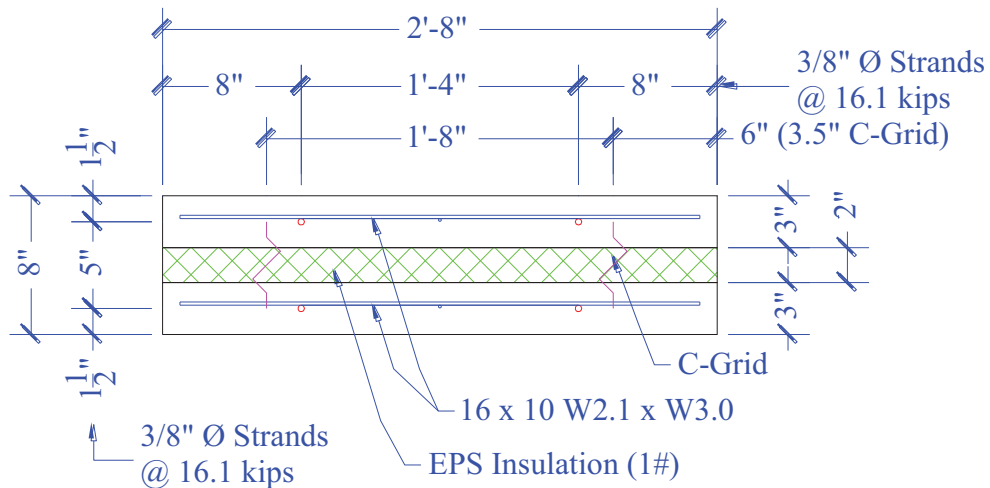
Figure 172. PCD2 Cross-Section Detail
