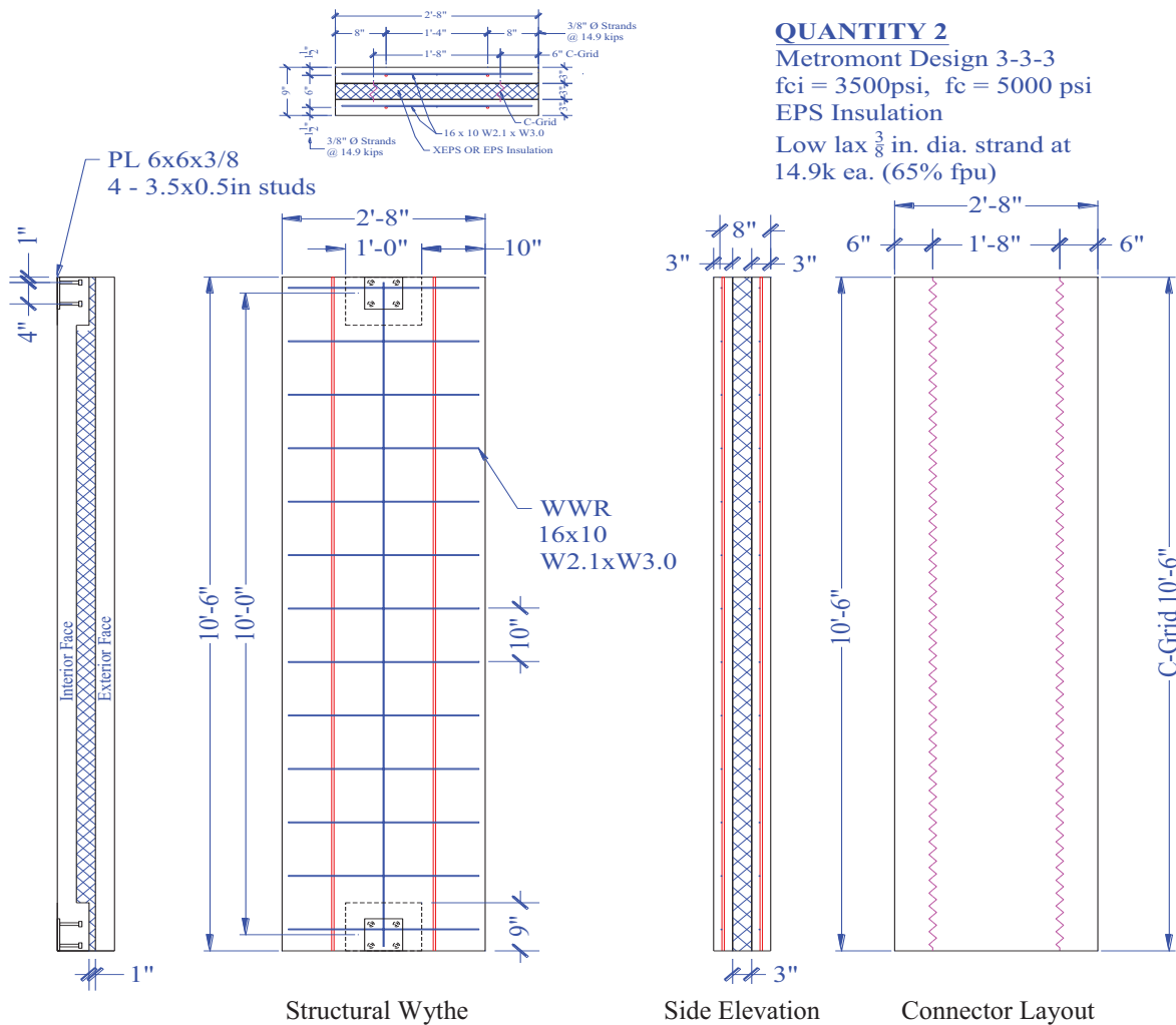
Figure 25. Specimen PCS10—Top Connection
