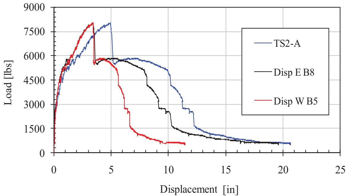
Figure 48. TS2-A Detail Results
