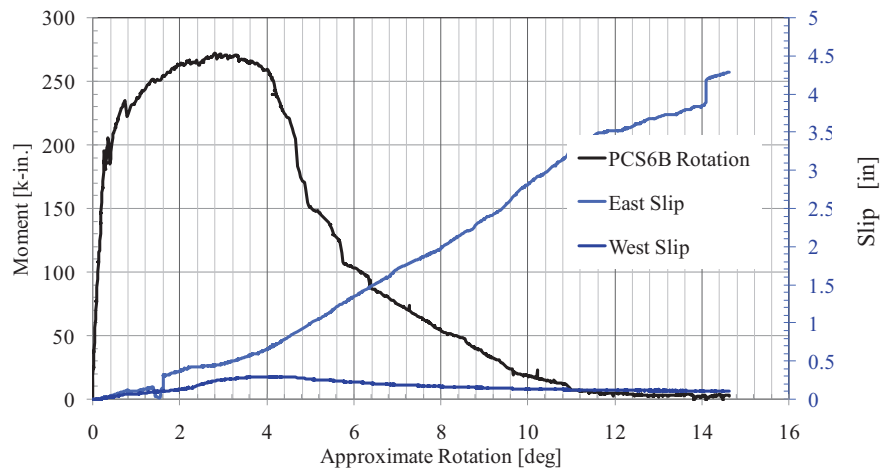
Figure 106. PCS6-B Response
