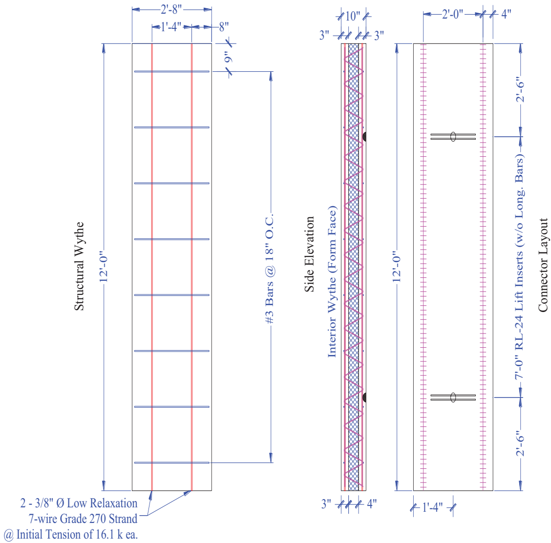
Figure 134. Tyn1 Panel Detail
