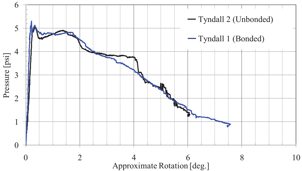
Figure 204. Average Single-span Response 3-4-3 Panels
