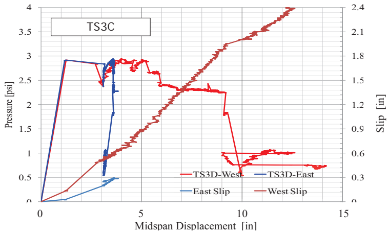
Figure 190. TS3-C, D Pressure-Displacement Response
