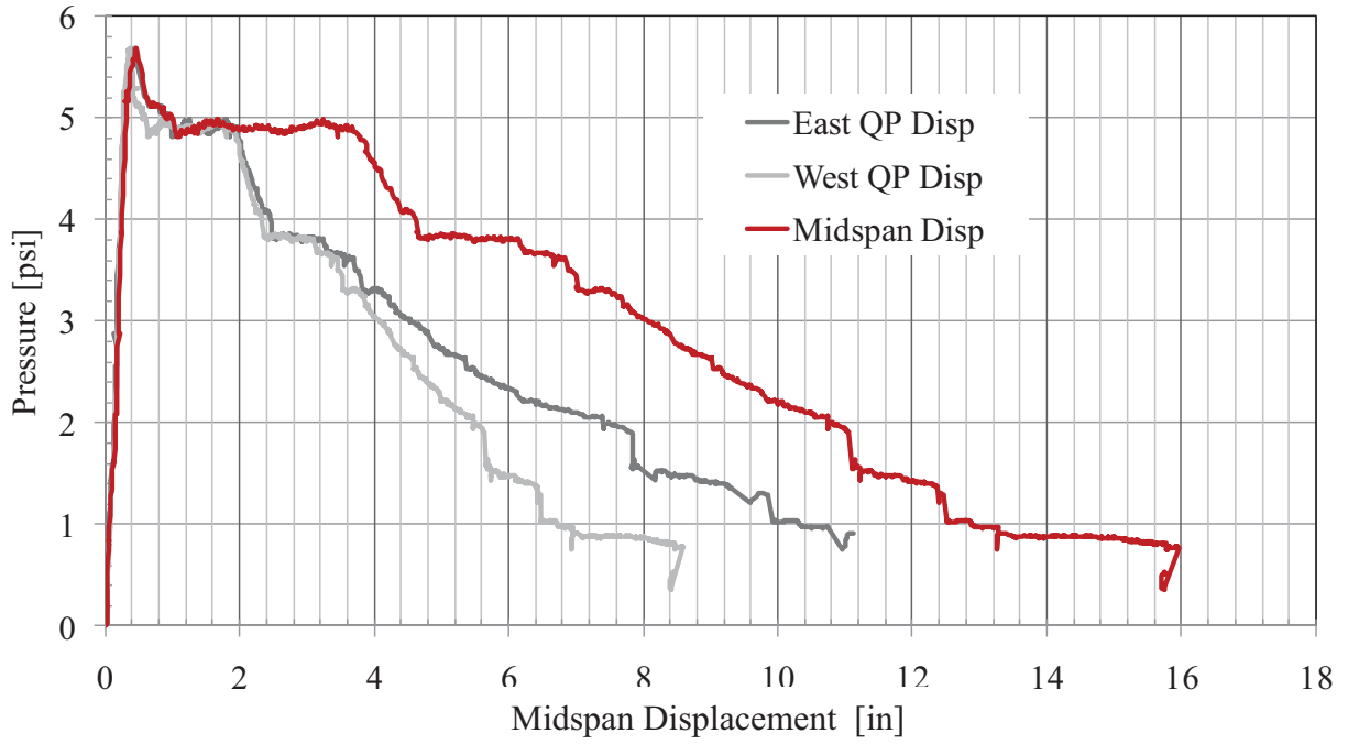
Figure 136. Tyn1-A Response
