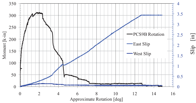
Figure 130. PCS9-B Response
