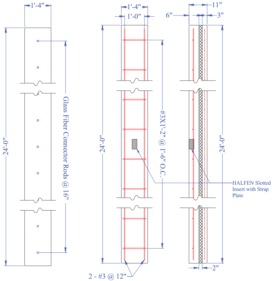
Figure 181. TS3-A, B Panel Detail
