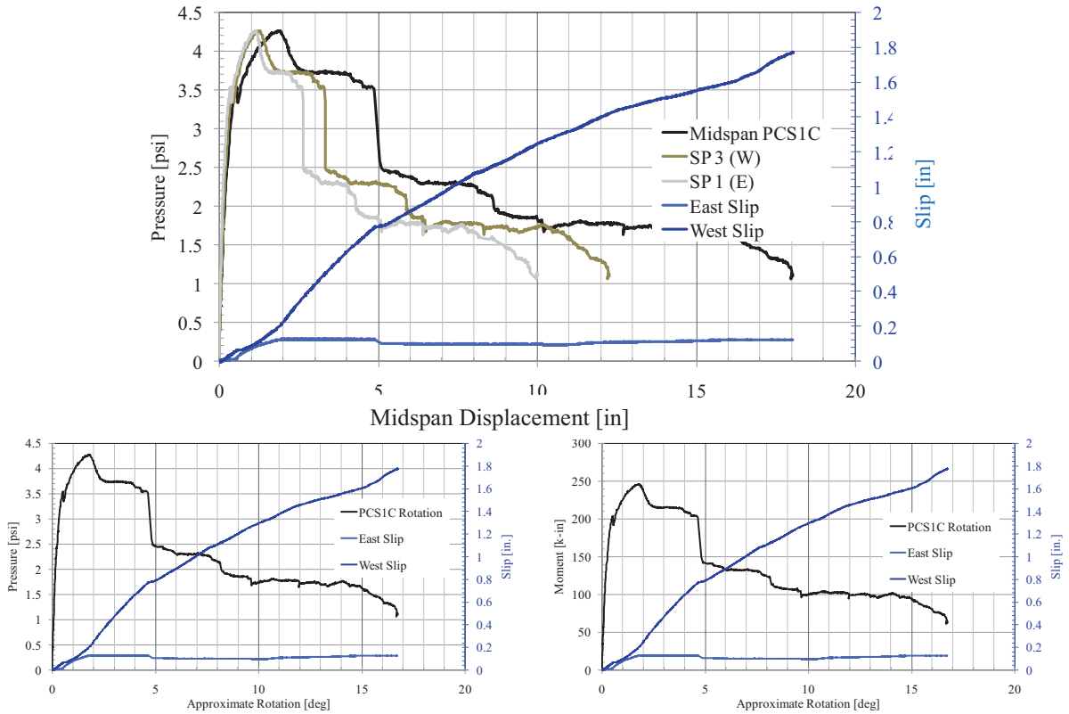
Figure 58. PCS1-C Response
