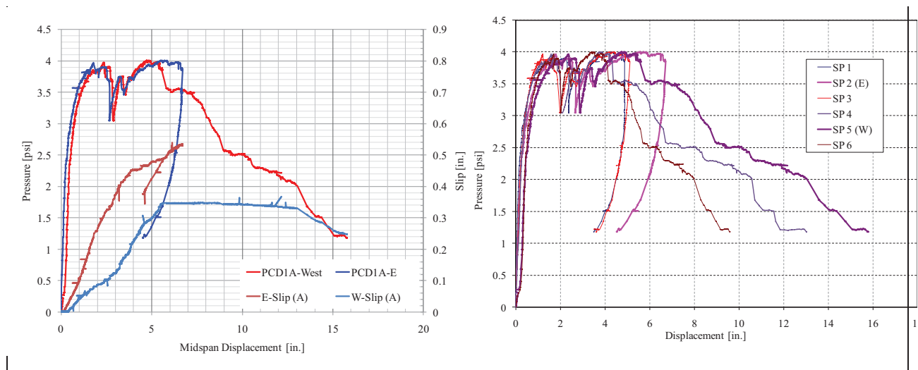
Figure 165. PCD1-A Response
