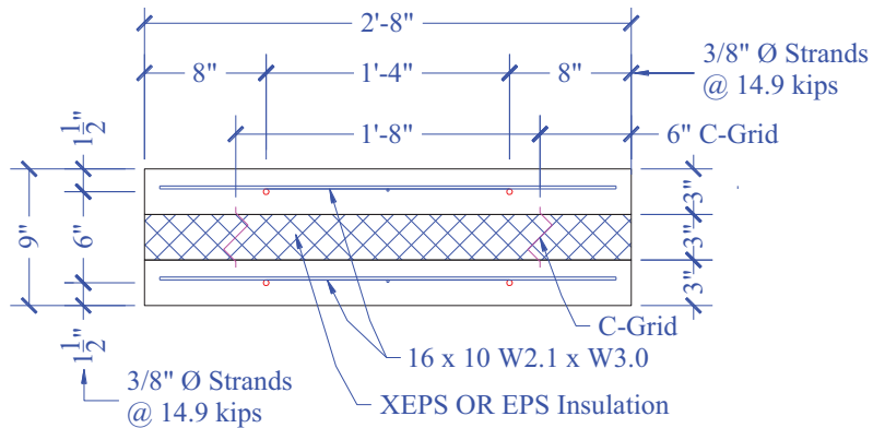
Figure 153. PCS11 Cross-Section Detail
