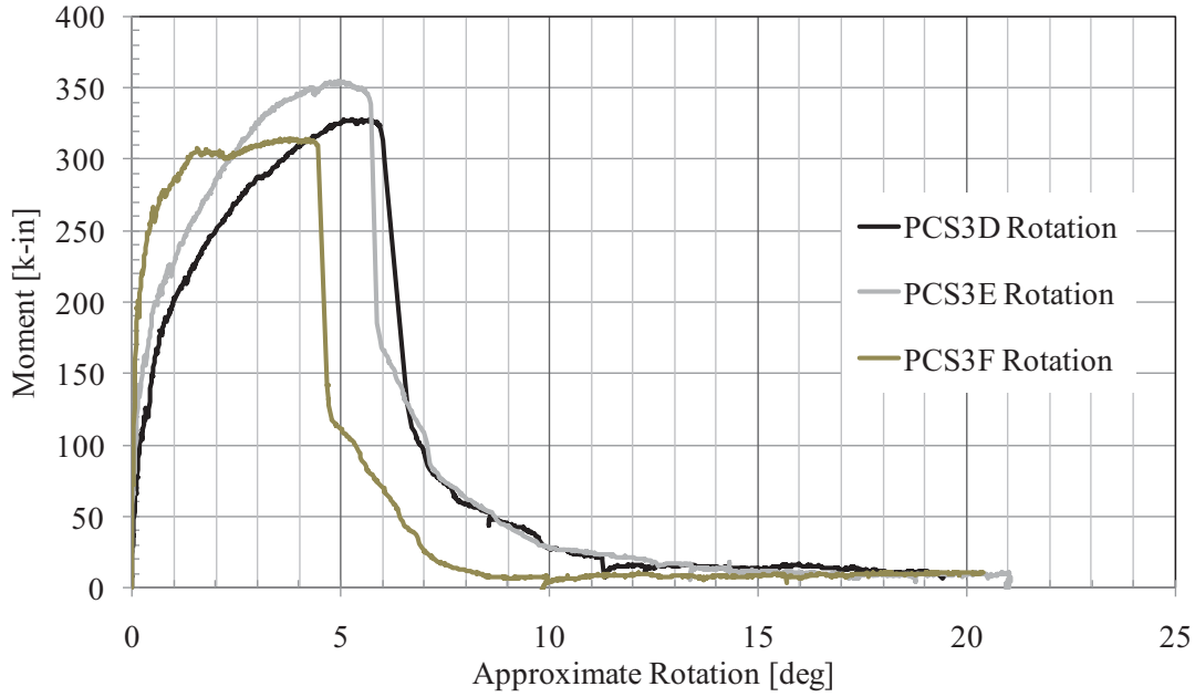
Figure 79. PCS3 (Type 2) Moment-Rotation Response
