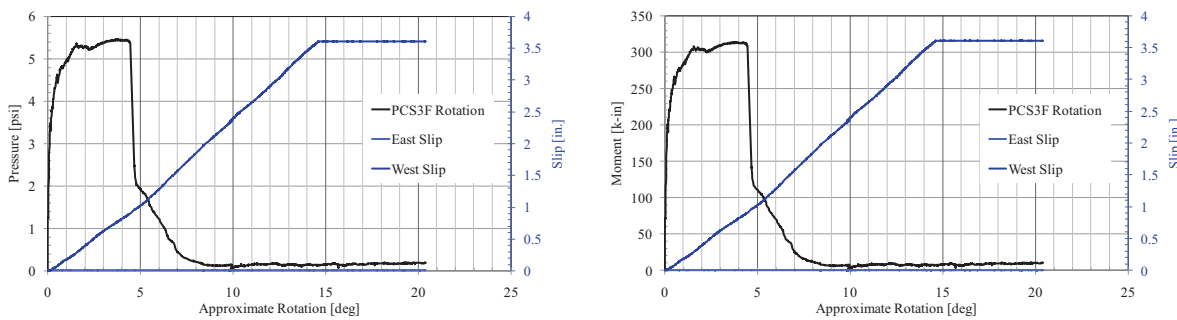
Figure 82. PCS3-F Response
