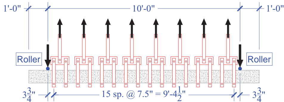
Figure 32. Single-span Loading Tree Schematic
