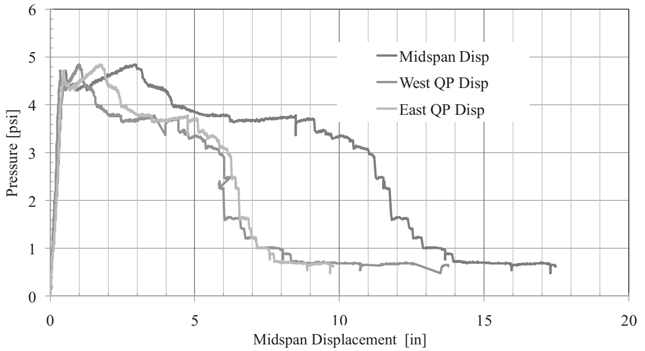
Figure 143. Tyn2-B Response
