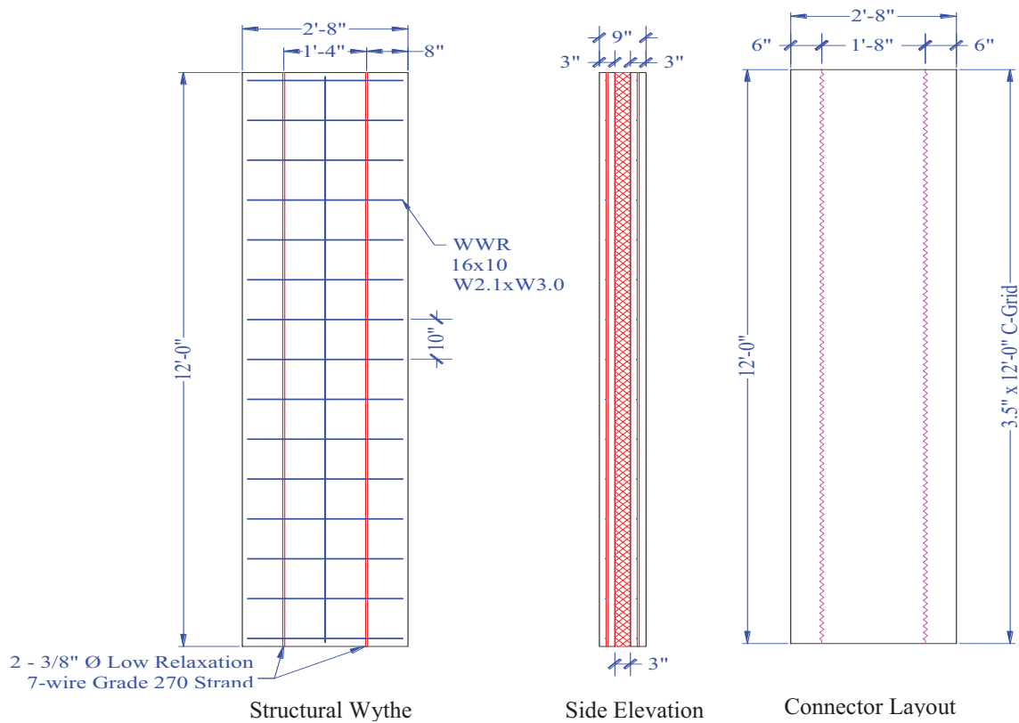
Figure 126. PCS9 Panel Detail
