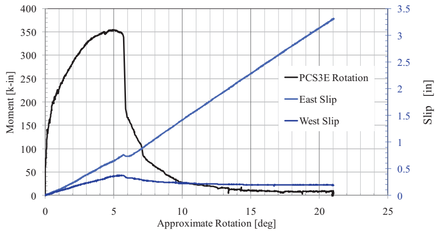
Figure 81. PCS3-E Response
