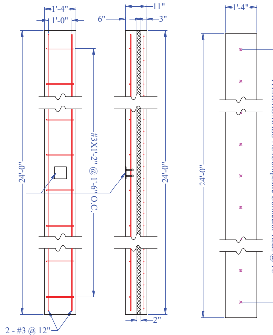
Figure 195. TS3-E, F Panel Detail
