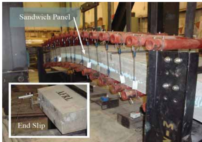
Figure 31. Single-span Loading Tree
