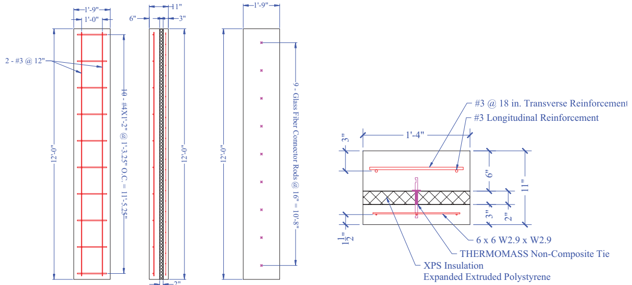
Figure 38. TS1 Reinforcement Details
